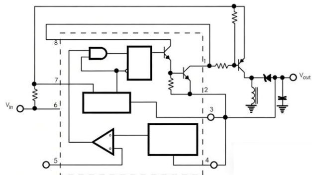
Fig6-b External PNP Saturated Switch
