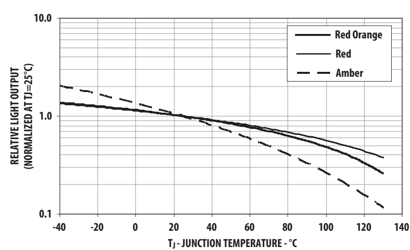
Figure 10: Relative Light Output vs. Junction Temperature
