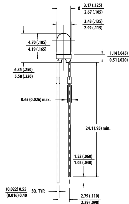
Figure 3: Package Outline “C” HLMP-1340/1440/1540/K640
