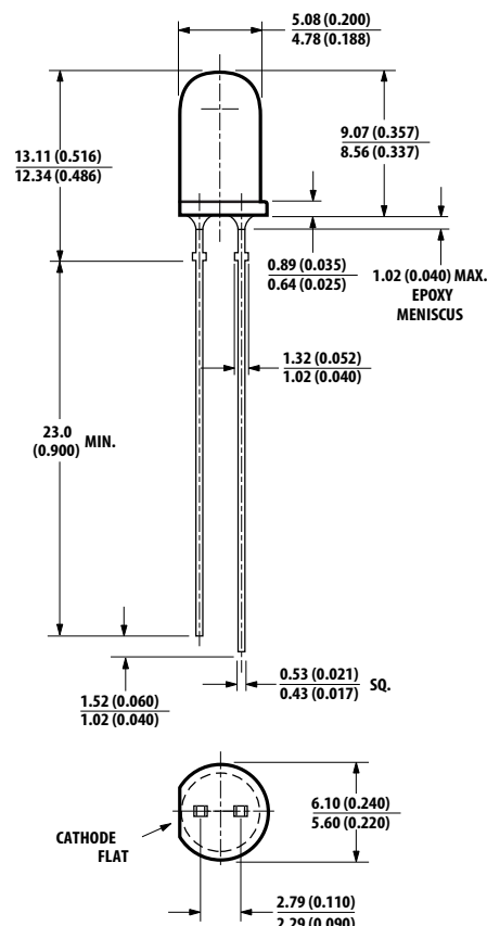
Figure 6: Package Outline “F” HLMP-3707/3907
