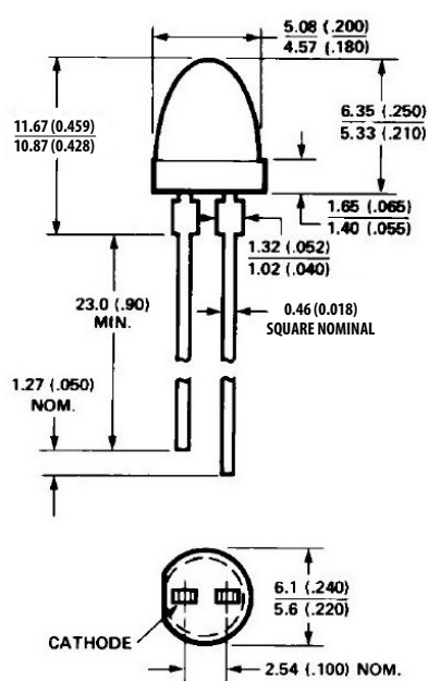
Figure 2: Package Outline “B” HLMP-3390/3490/3590
