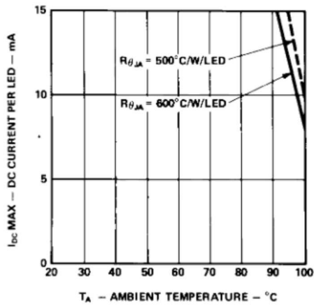
Figure 2. Maximum Allowed DC Current per LED vs. Ambient Temperature, T_{J\text{MAX}} = 110^{\circ}\text{C} .
