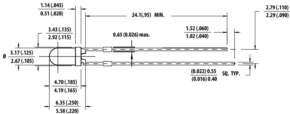
Figure 2: T-1¼ Package
