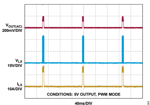
Figure 43. Overload Protection (Figure 54 Circuit)
