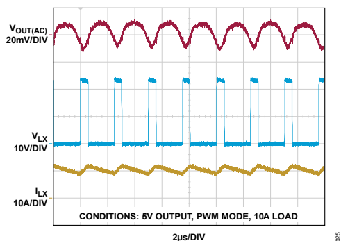
Figure 25. Steady-State Performance (Figure 54 Circuit)
