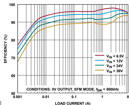
Figure 10. Efficiency vs. Load Current (Figure 56 Circuit)
