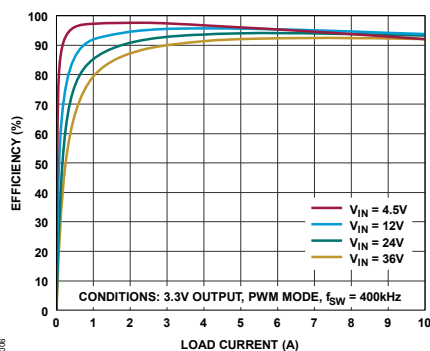
Figure 7. Efficiency vs. Load Current (Figure 55 Circuit)
