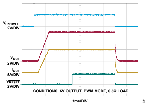
Figure 21. Soft-Start/Shutdown Through EN/UVLO (Figure 54 Circuit)
