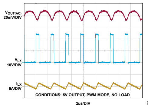
Figure 26. Steady-State Performance (Figure 54 Circuit)
