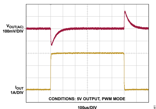
Figure 41. Load Transient Between 10mA and 3A (Figure 57 Circuit)
