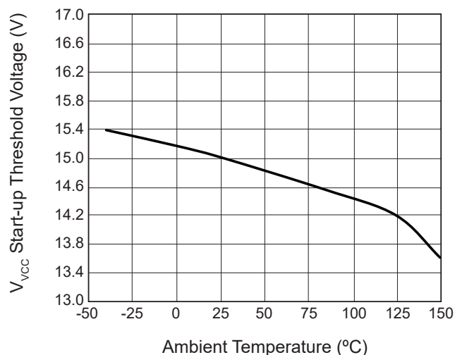
Figure 7. V_{VCC} Start-up Threshold Voltage vs. Ambient Temperature
