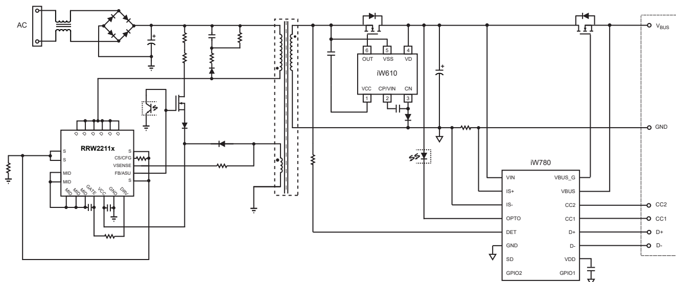
Figure 2. RRW2211x Typical Application Circuit with Active Start-up Circuit (Using iW780 as Secondary-Side Controller and iW610 as top side SR controller Achieving Multi-Level CV/CC Regulation and < 5mW Standby Power Consumption at 230V AC )
