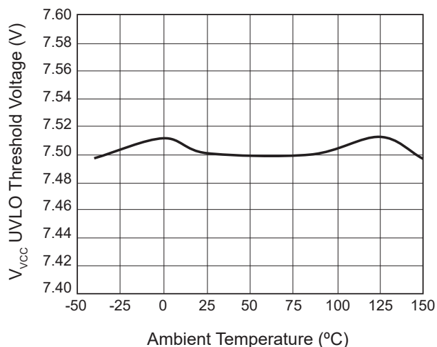
Figure 8. V_{VCC} Start-up Threshold Voltage vs. Ambient Temperature
