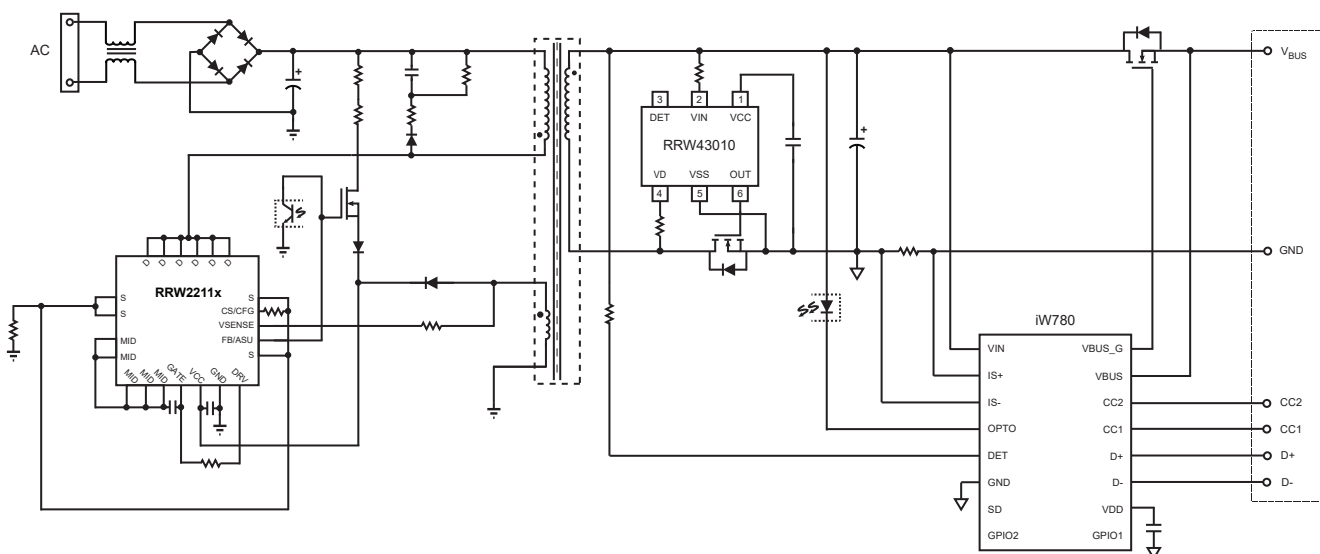
Figure 3. RRW2211x Typical Application Circuit with Active Start-up Circuit (Using iW780 as Secondary-Side Controller and RRW43010 as low side SR controller Achieving Multi-Level CV/CC Regulation and < 5mW Standby Power Consumption at 230V AC )
