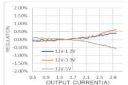
Load Regulation
