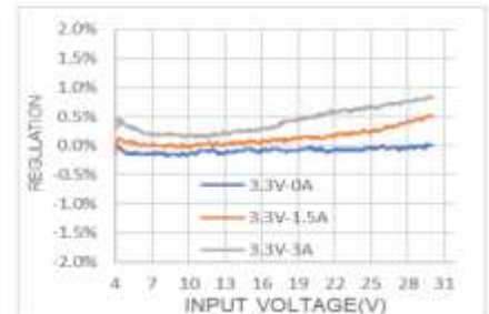
Line Regulation
