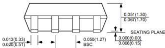
FRONT VIEW
