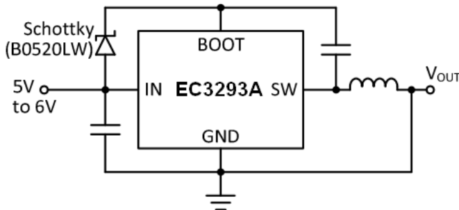
Figure 3: Add a Schottky diode to promote efficiency when V_{IN} \leq 6\text{V} .
