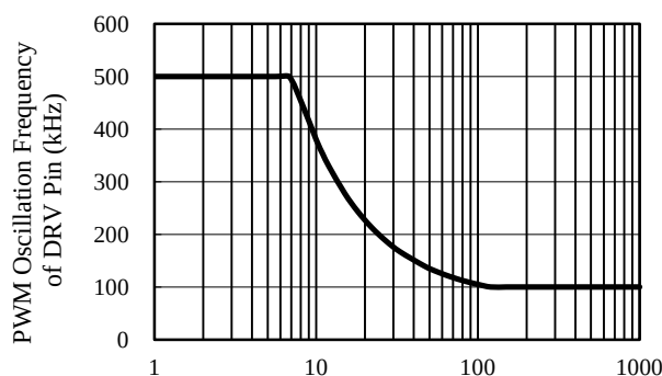
Figure 8-9. Relation between PWM Oscillation Frequency and R_{FSET}
