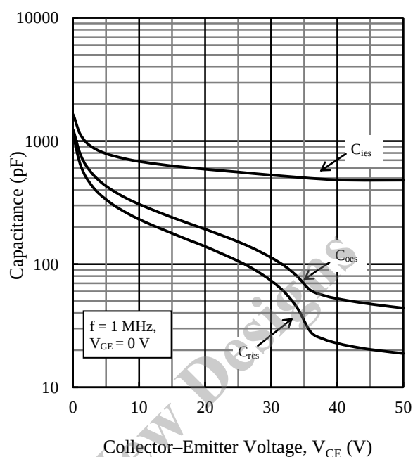
Figure 13. Capacitance Characteristics
