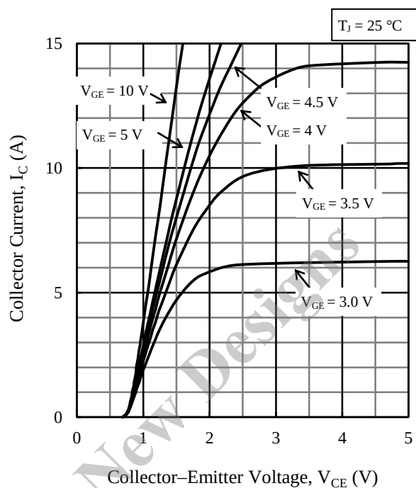
Figure 5. Output Characteristics ( T_J = 25\text{ }^{\circ}\text{C} )
