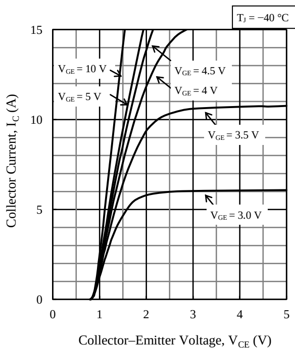
Figure 4. Output Characteristics ( T_J = -40\text{ }^{\circ}\text{C} )
