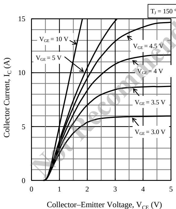
Figure 6. Output Characteristics ( T_J = 150\text{ }^{\circ}\text{C} )
