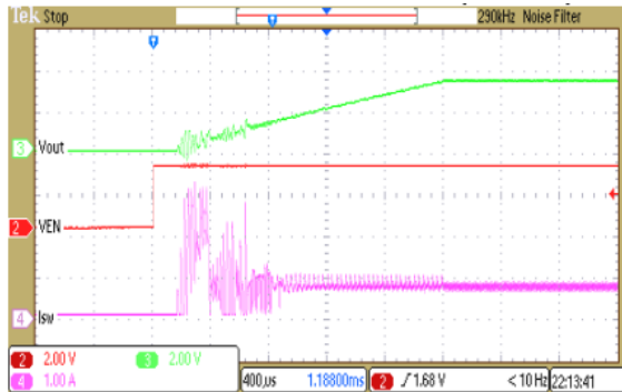
Start UP & Inrush Current 12V→3.3V (Load 1A)
