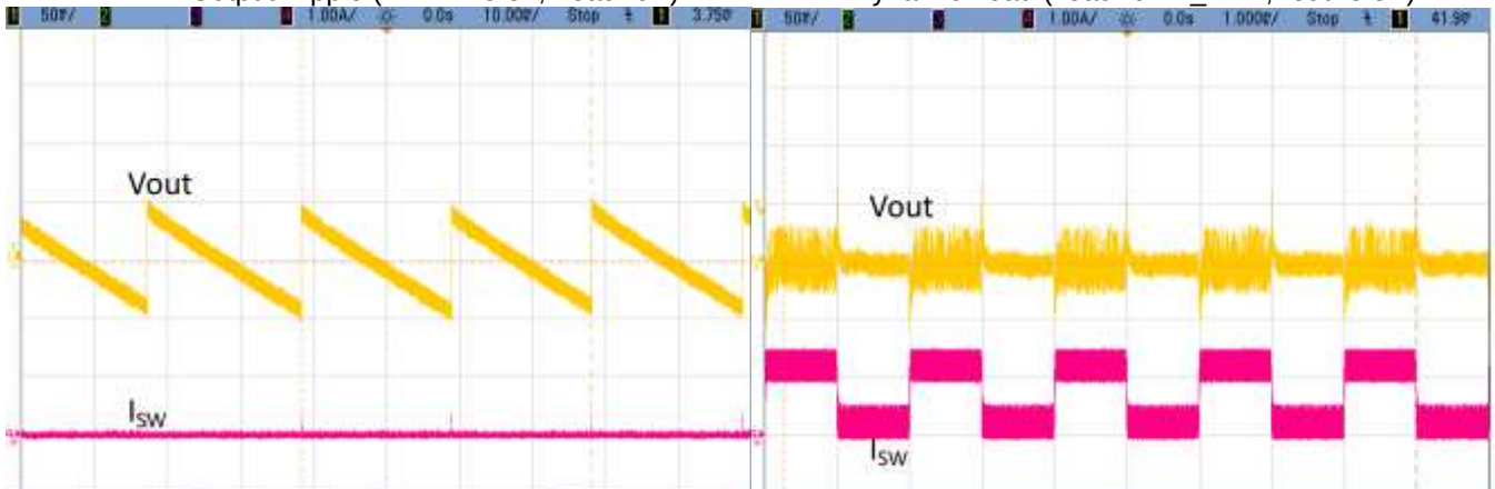
Output Ripple (12V => 3.3V, Load=0A)
