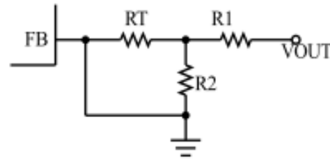
Figure 1 : T-type network
