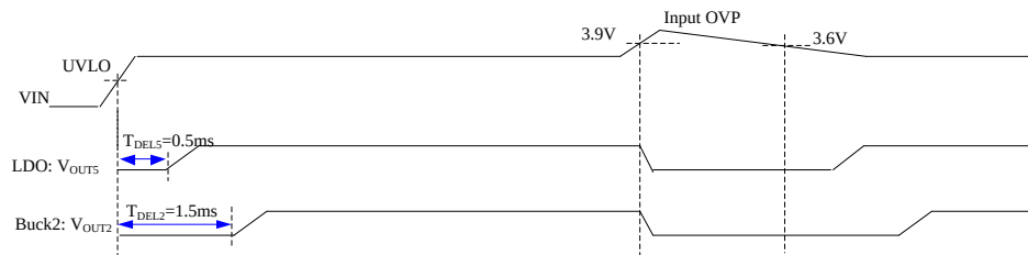
Figure 9. Input over voltage protection
