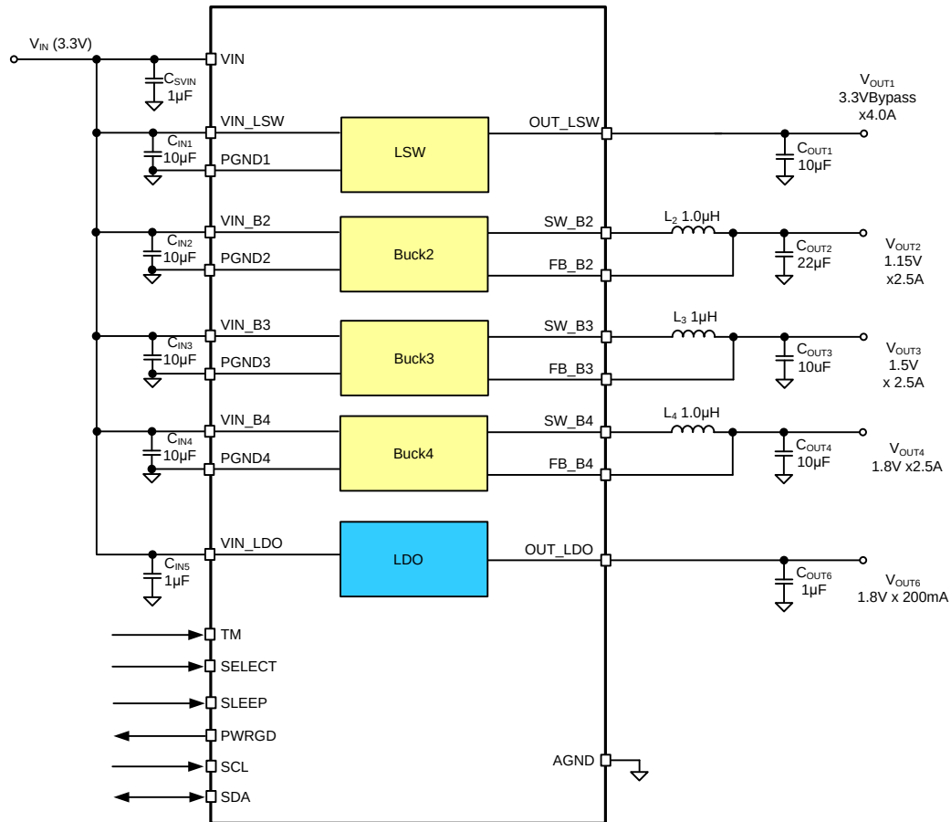
Figure1. Schematic Diagram
