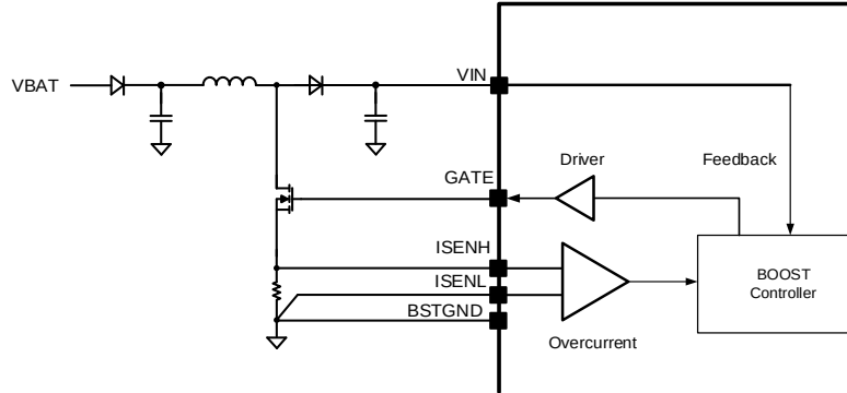
Figure 7. Boost Regulator
