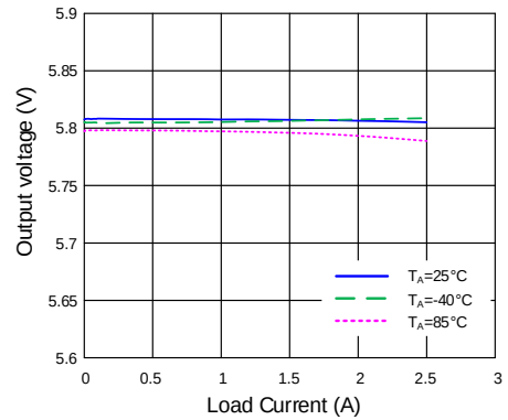
VOPRE Buck Output Voltage vs Load Current (VIN=12V, FSW Pin Open, Fre=2.2MHz)
