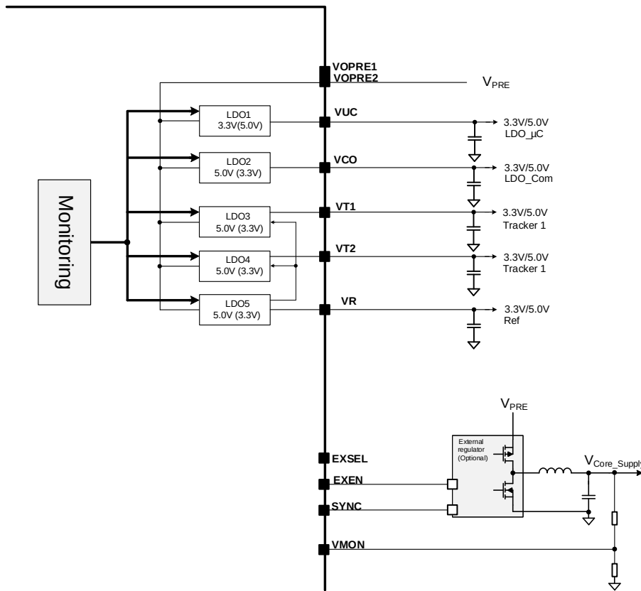
Figure 9. Post Regulators
