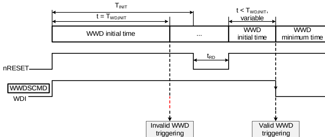
Figure 49. Incorrect Timing: No Trigger within Initial Time ( T_{WD,INIT} < T_{SYS,INIT} )
