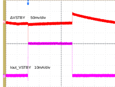
VSTBY Dynamic Load Response(0mA to 30mA) (FSW-Pin: Open; VSTBY=5V; C vstby =4.7μF)
