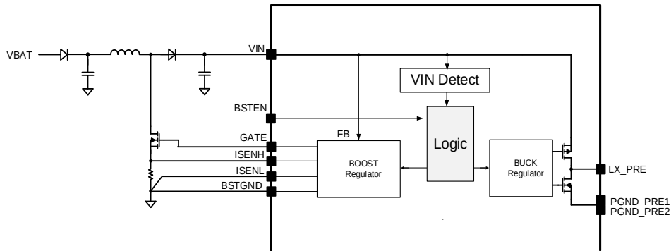
Figure 6. Pre-regulator Stage Block Diagram
