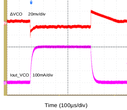
VCO Dynamic Load Response(1mA to 300mA) (FSW-Pin: Open; VCO=3.3V; C VCO =11μF)
