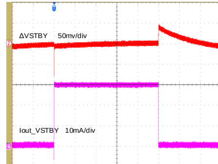
VSTBY Dynamic Load Response(0mA to 30mA) (FSW-Pin: Open; VSTBY=3.3V; C vstby =4.7μF)
