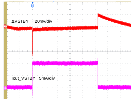
VSTBY Dynamic Load Response(0mA to 10mA) (FSW-Pin: Open; VSTBY=3.3V; C vstby =4.7μF)
