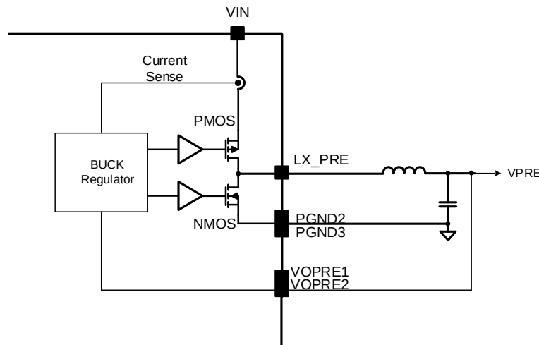
Figure 8. Buck Regulator
