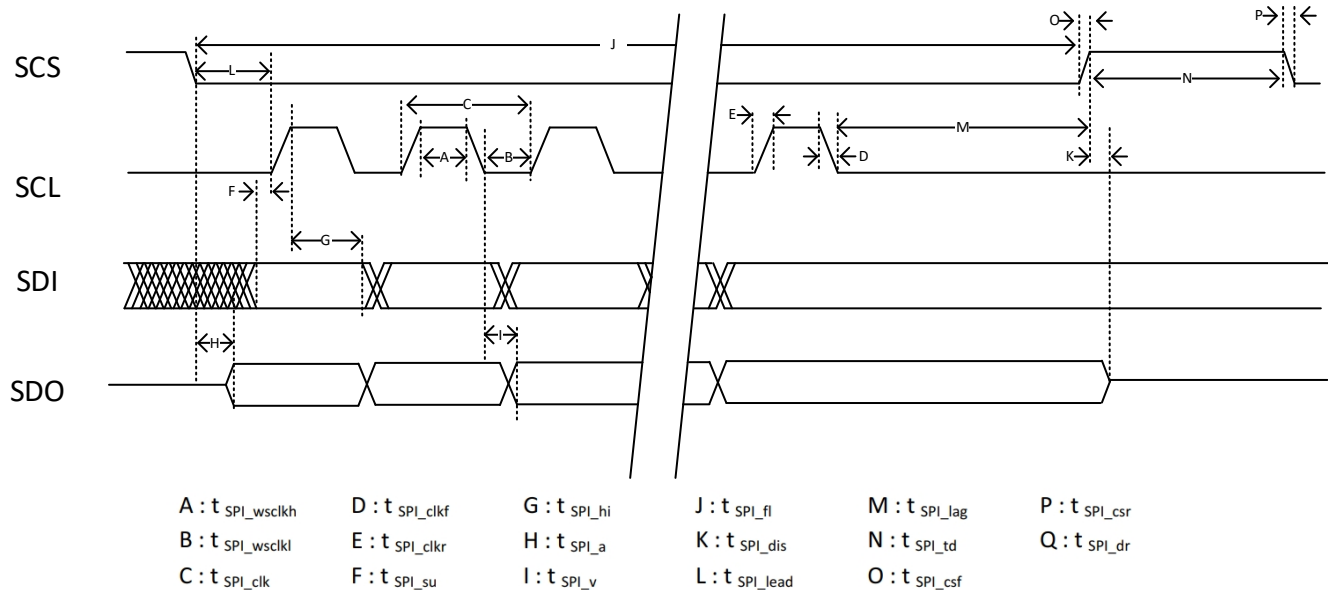
Figure 73. SPI Timing
