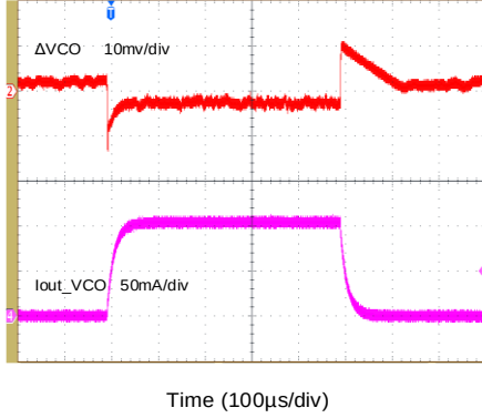
VCO Dynamic Load Response(1mA to 100mA) (FSW-Pin: Open; VCO=3.3V; C VCO =11μF)
