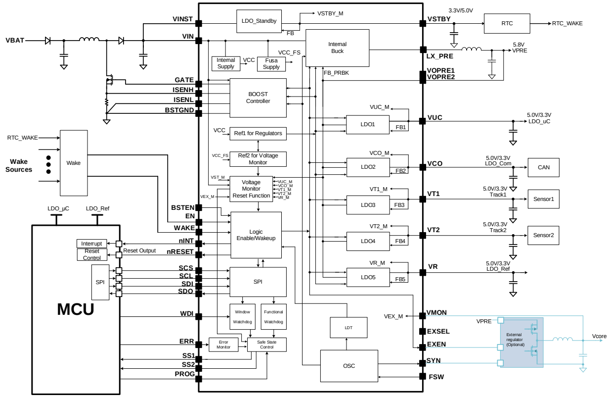
Figure 1. Application Schematic
