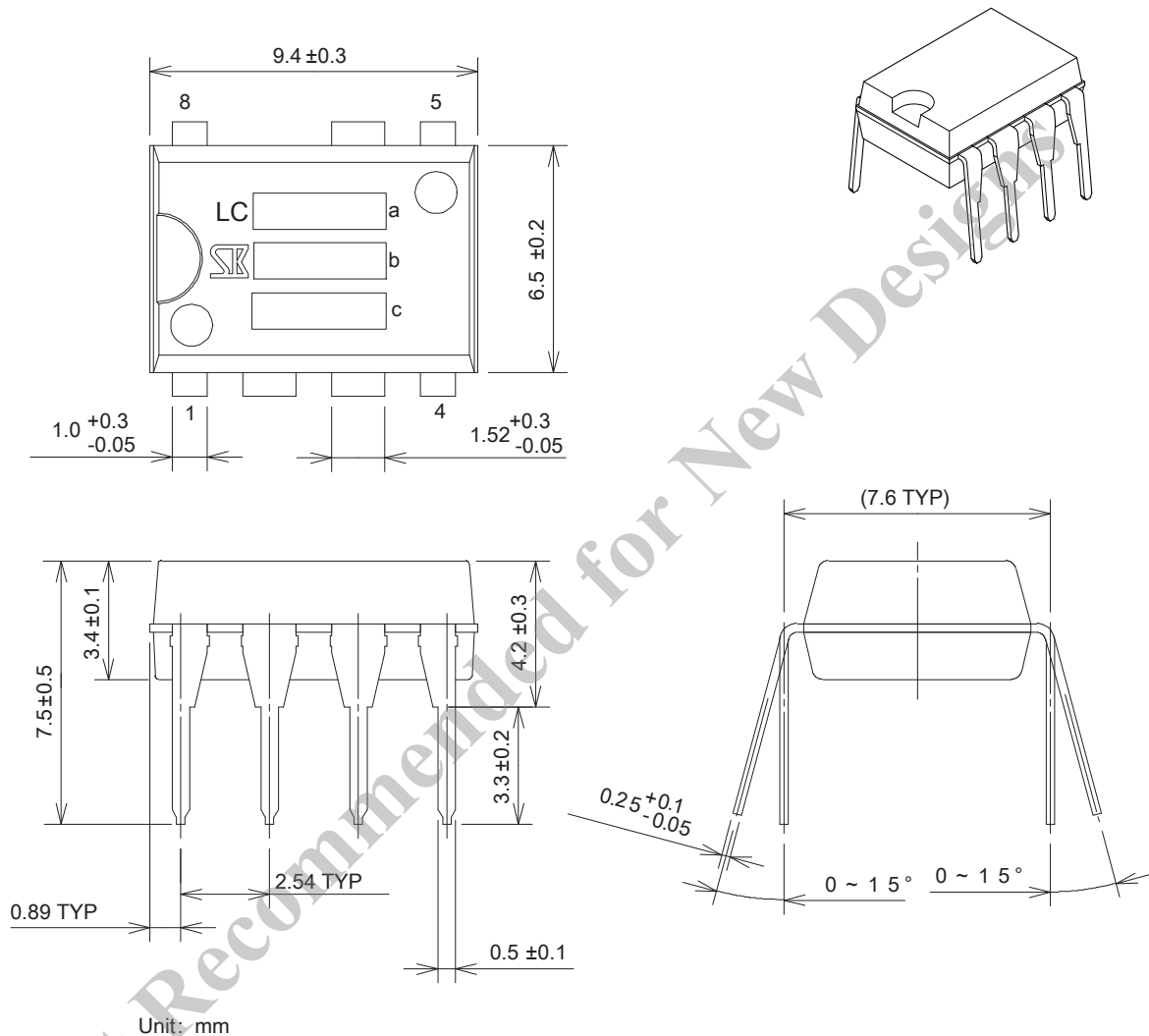
Package Outline Drawing, DIP8
