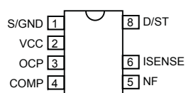
Pin-out Diagram
