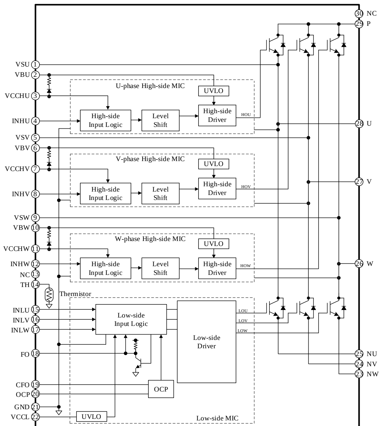
Figure 8-1. Block Diagram
