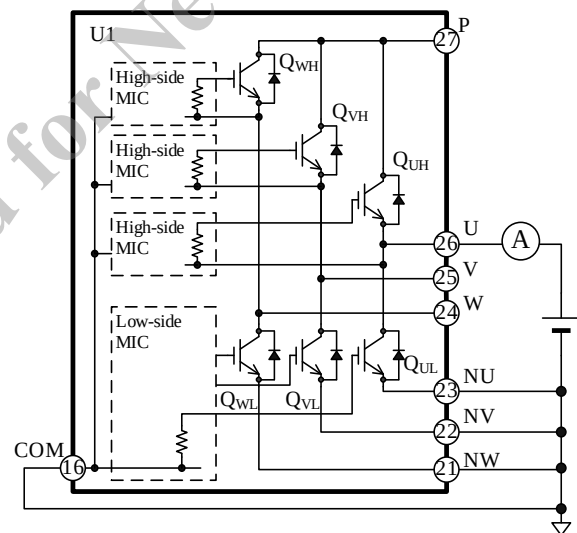
Figure 14-4. Typical Measurement Circuit for Low-side IGBT ( Q_{III} ) in U-phase
