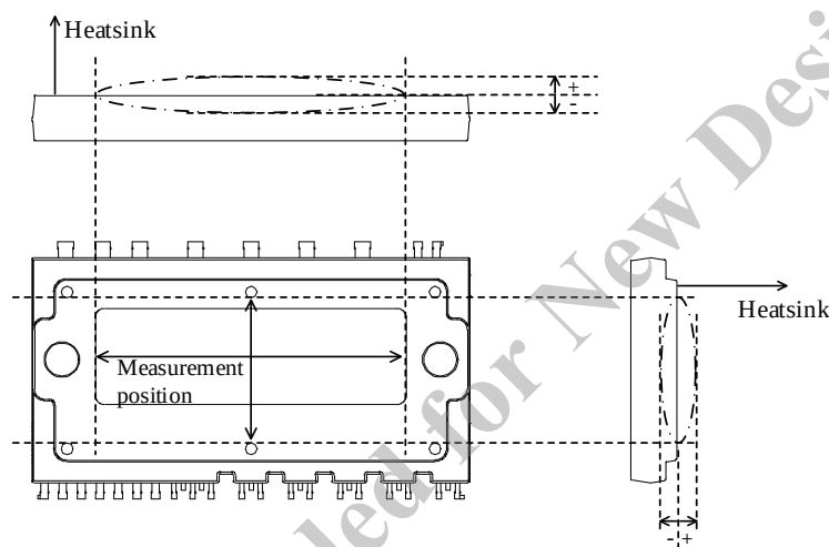
Figure 5-1. Flatness Measurement Position
