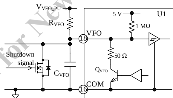
Figure 13-9. Internal Circuit Diagram of VFO Pin and Its Peripheral Circuit
