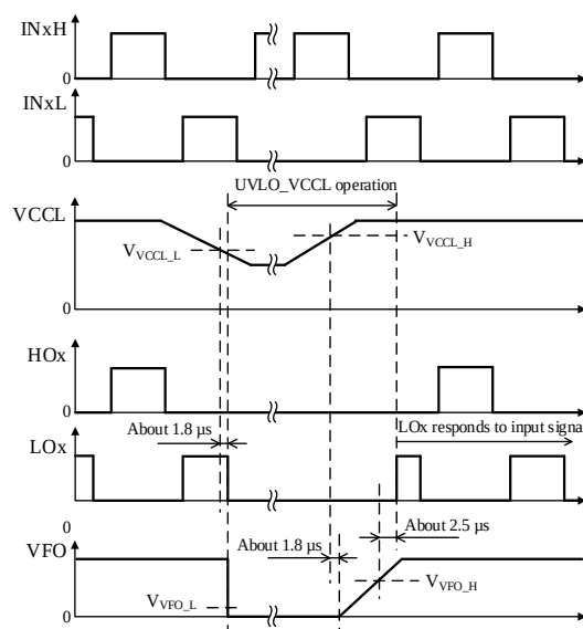
Figure 13-12. UVLO_VCCL Operational Waveforms
