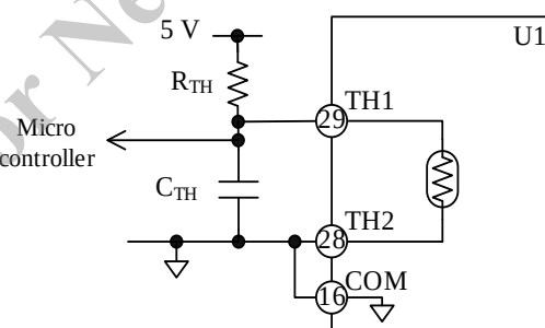
Figure 13-6. When Output Voltage Has Negative Temperature Characteristic
