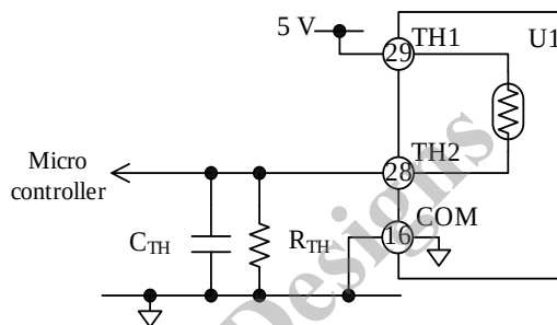
Figure 13-5. When Output Voltage Has Positive Temperature Characteristic
