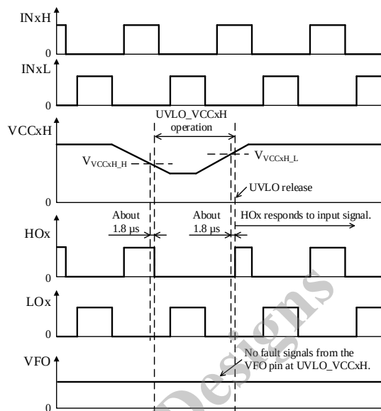
Figure 13-11. UVLO_VCCxH Operational Waveforms
