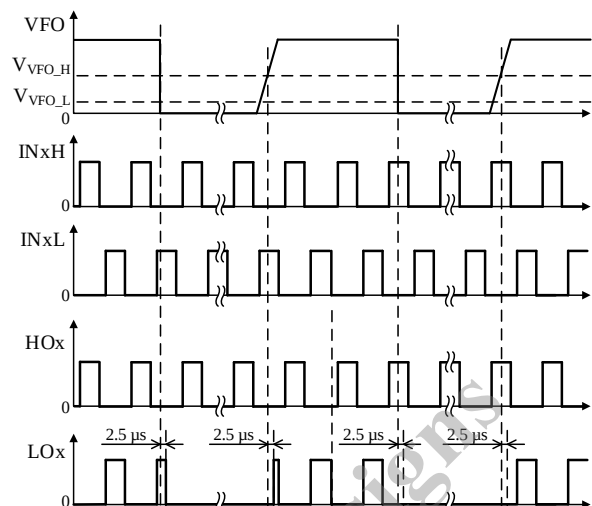
Figure 13-8. Operational Waveforms of Shutdown Signal Input
