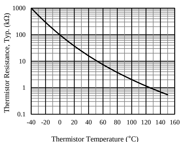
Figure 13-7. Typical Thermistor Resistance vs. Temperature Curve
