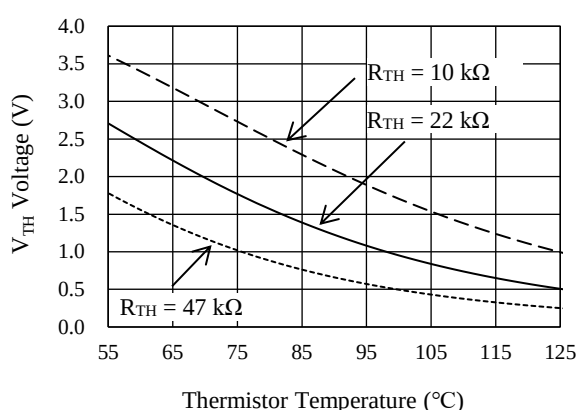
Figure 14-10. V_{TH} Voltage vs. Thermistor Temperature ( V_{TH\_PU} = 5.0 V)
