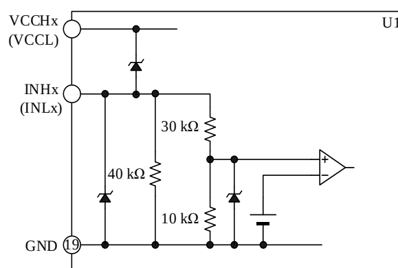
Figure 14-5. Internal Circuit Diagram of INHx or INLx Pin
