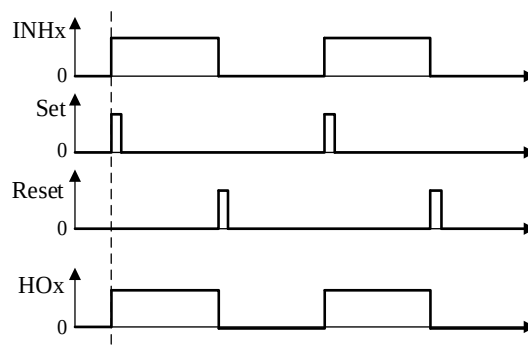
Figure 14-3. Operational Waveforms of Level-shifting Circuit
