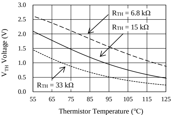
Figure 14-9. V_{TH} Voltage vs. Thermistor Temperature ( V_{TH\_PU} = 3.3 V)
