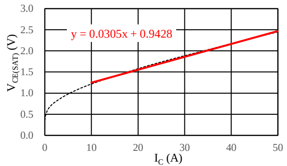
Figure 16-1. Linear Approximate Equation of V_{CE(SAT)} vs. I_C
