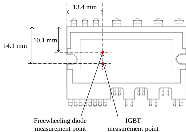
Figure 5-4. SAM470M30AF1 Case Temperature Measurement Point
