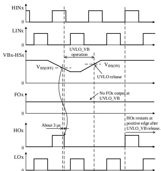
Figure 12-16. UVLO_VB Operational Waveforms
