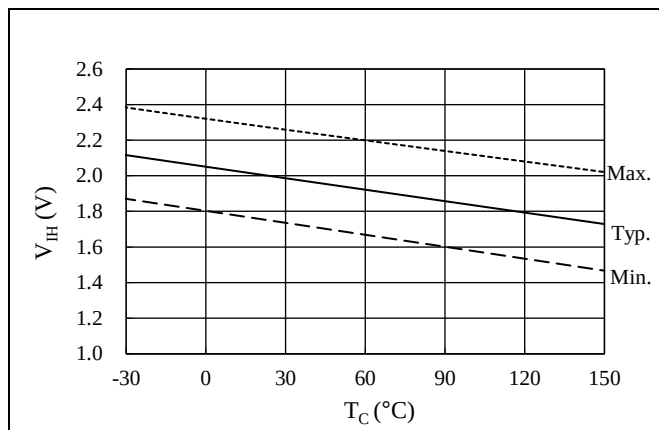
Figure 15-14. High Level Input Signal Threshold Voltage, V_{IH} vs. T_C
