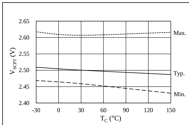
Figure 15-20. SCP Threshold Voltage, V_{SCPT} vs. T_C
