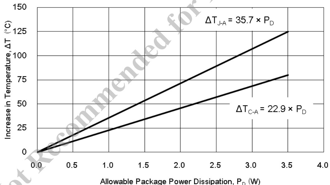
Figure 14-1. Temperature Increase
