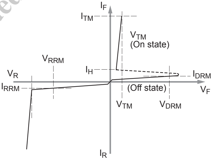
Voltage-Current Characteristic
