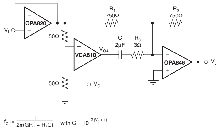
Figure 43. Tunable Equalizer
