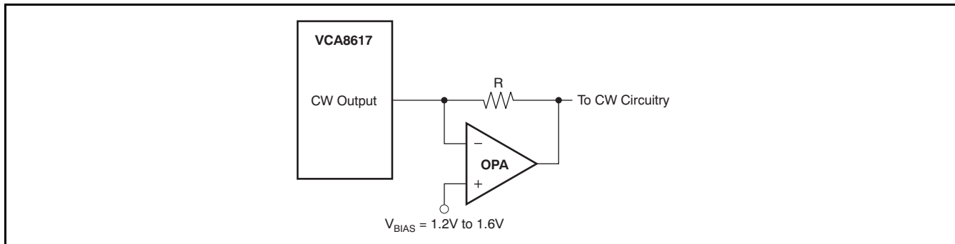
Figure 63. Operational Amplifier
