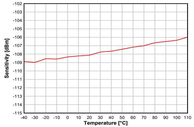
Figure 8-13. Sensitivity vs. Temperature (50 kbps, 868.3 MHz)
