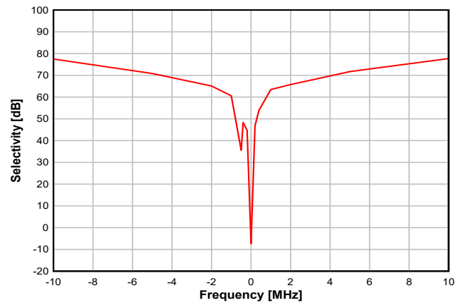
Figure 8-15. Selectivity vs. Frequency Offset (50 kbps, 868.3 MHz)
