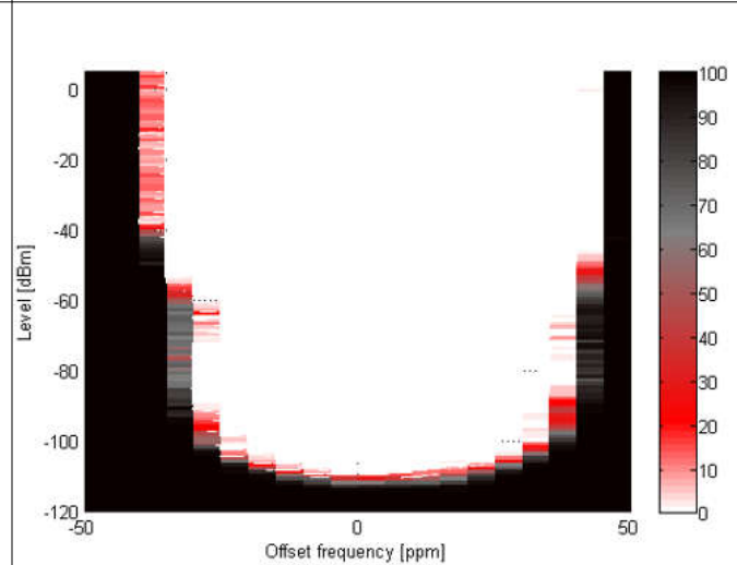
Figure 8-17. 802.15.4, 50 kbps, ±25 kHz deviation, 2-GFSK, 100 kHz RX Bandwidth
