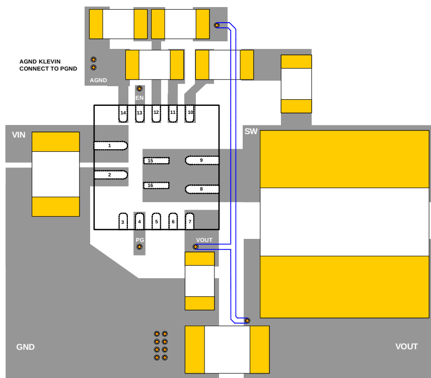
Figure 15: Recommend Layout
