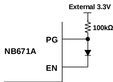
Figure 13: PG Pull up to external power supply with enable control signal --- Single PG Output
