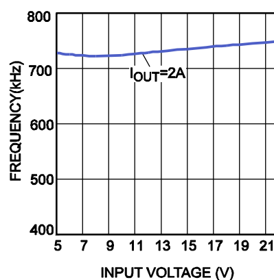
Switch Frequency vs. Input Voltage
