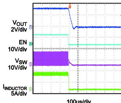
Enable Shutdown with 7A load
