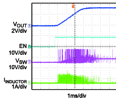
Enable Startup without Load
