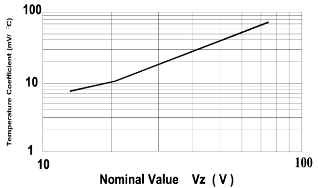
Fig 2. Temperature Coefficient
