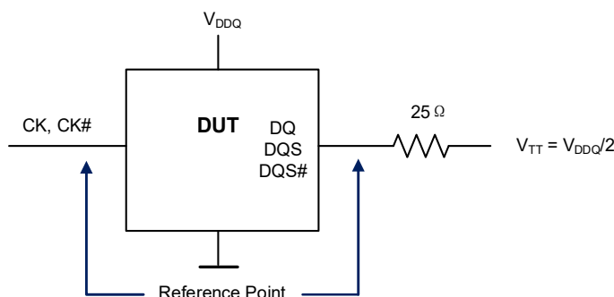
Figure 8-3. Reference Load for AC Timing and Output Slew Rate
