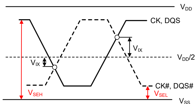
Figure 7-4. V_{IX} Definition
