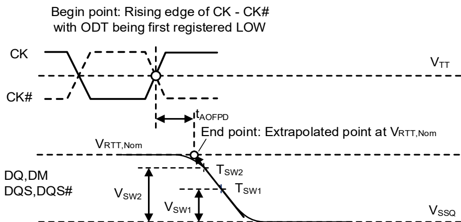
Figure 8-12. Definition of t_{AOFDPD}
