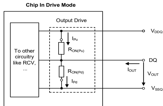
Figure 8-6. Output Driver: Definition of Voltages and Currents
