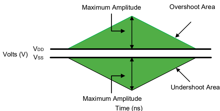
Figure 8-4. Address and Control Overshoot and Undershoot Definition
