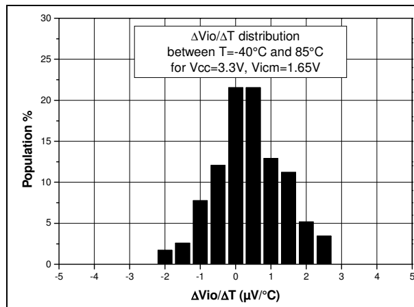
Figure 8. Input offset voltage temperature coefficient distribution
