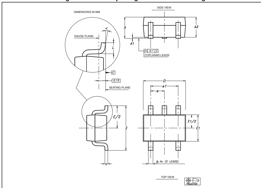
Figure 42. SC70-5 package mechanical drawing
