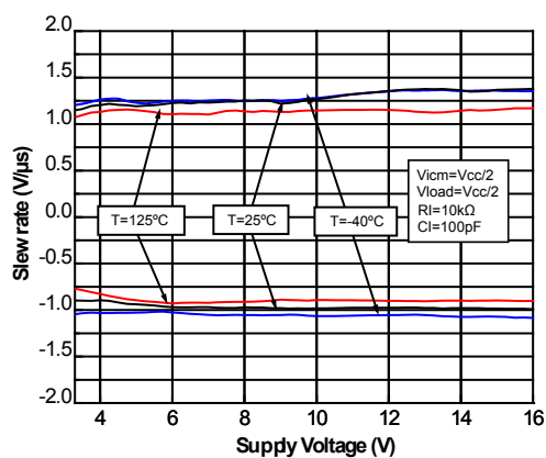
Figure 17. Slew rate vs. supply voltage
