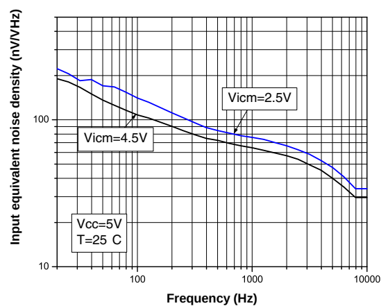
Figure 12. Noise vs. frequency
