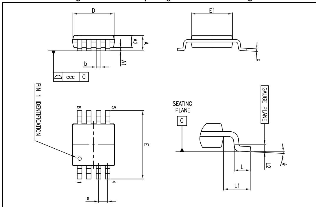
Figure 25. MiniSO-8 package mechanical drawing
