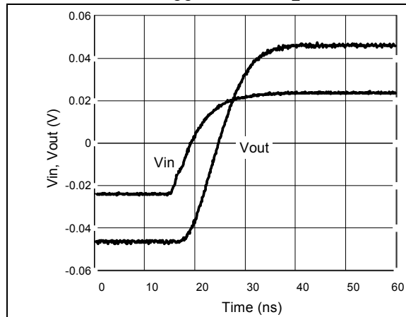
Figure 23. Small signal measurement - rise time (gain = 2, V_{CC} = \pm 2.5\text{ V} , Z_L = 150\ \Omega )
