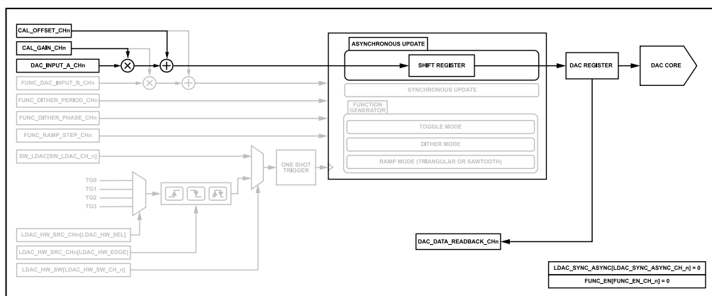
Figure 44. Asynchronous Block Diagram
