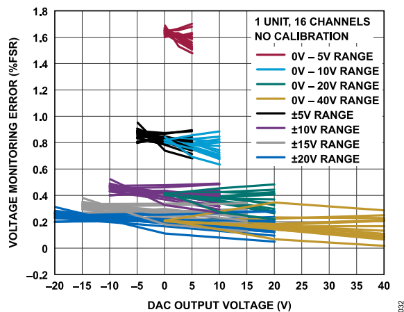
Figure 32. DAC Output Voltage Monitoring Error vs. DAC Output Voltage, No Calibration
