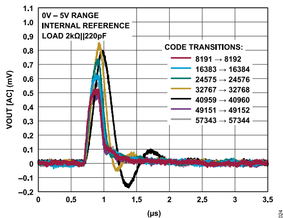
Figure 24. Glitch Amplitude, 0V to 5V Range
