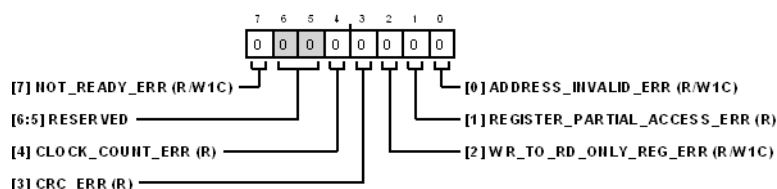
Figure 86. Interface Status A Register
