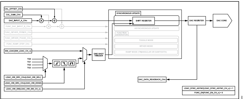
Figure 43. Synchronous Block Diagram
