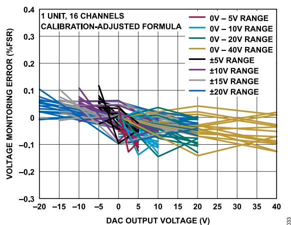
Figure 33. DAC Output Voltage Monitoring Error vs. DAC Output Voltage, Calibration-Adjusted Formula
