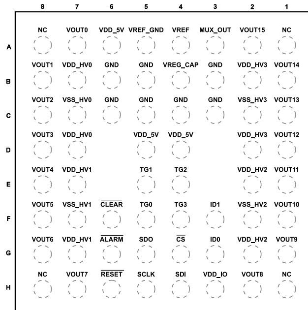
Figure 4. Pin Configuration
