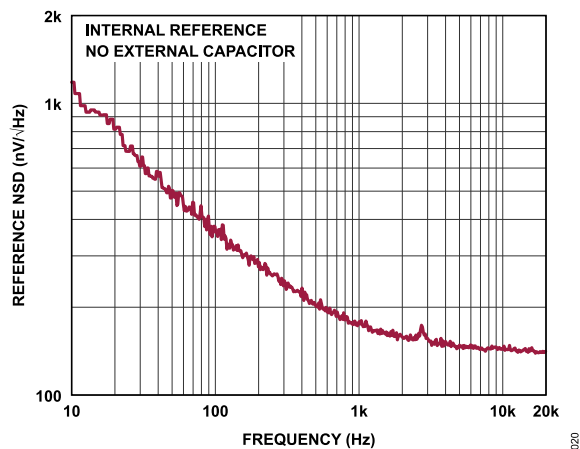
Figure 20. Internal Reference Noise Spectral Density
