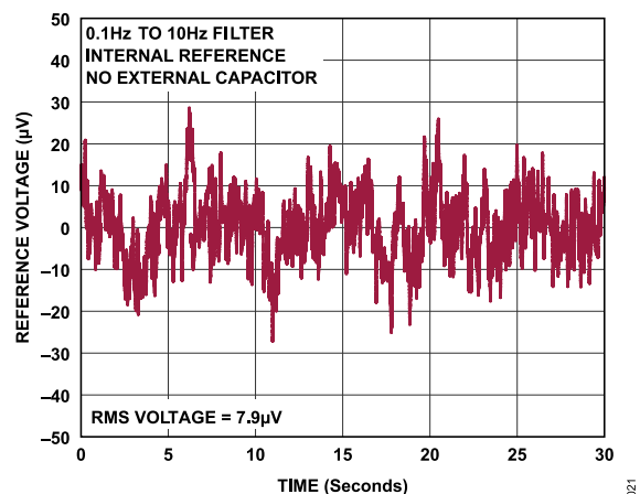
Figure 21. Internal Reference Noise
