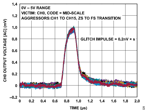
Figure 28. DAC-to-DAC Crosstalk
