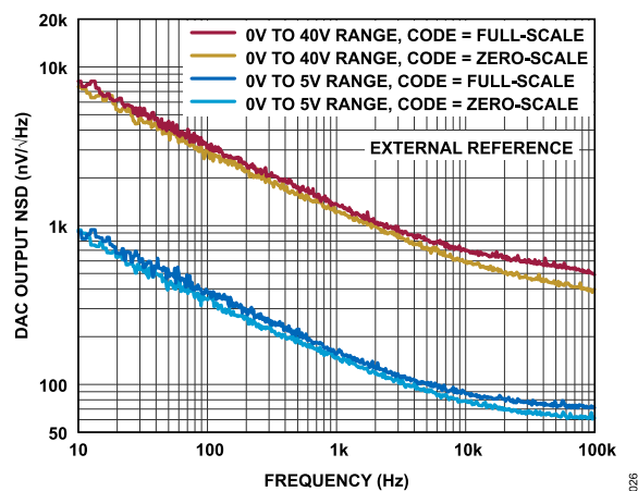
Figure 26. DAC Output Noise Spectral Density
