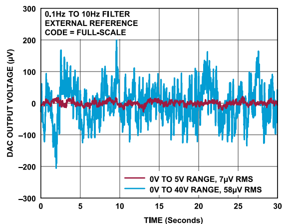
Figure 27. DAC Output Noise
