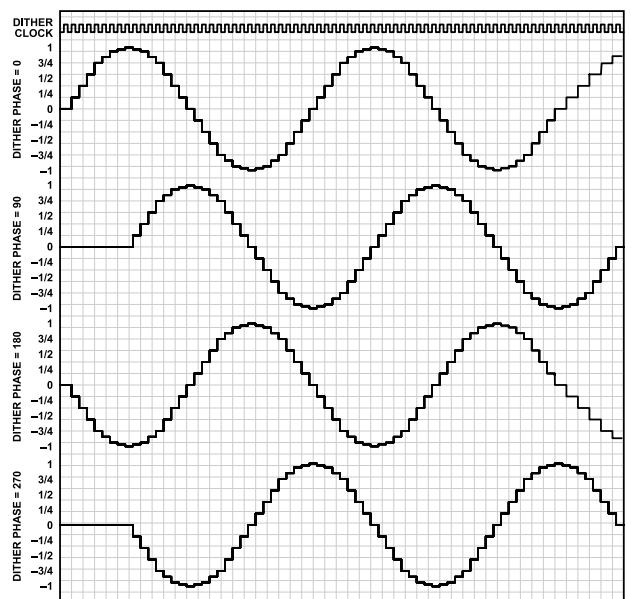
Figure 52. Dither Waveform for Different Values of \phi
