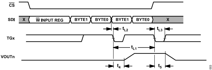
Figure 3. LDAC Timing
