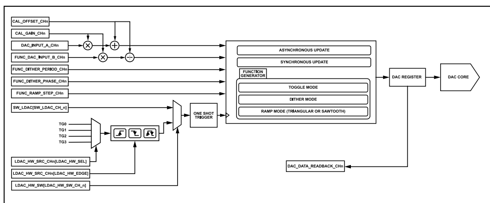
Figure 45. Digital Functions Diagram
