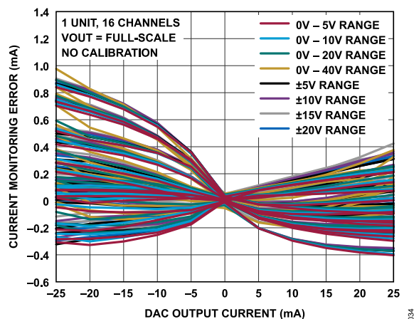
Figure 34. DAC Output Current Monitoring Error vs. DAC Output Current
