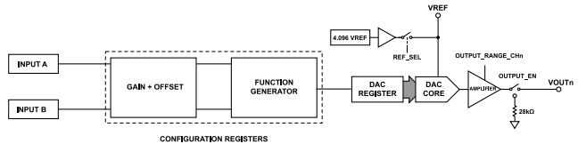
Figure 41. DAC Channel Block Diagram
