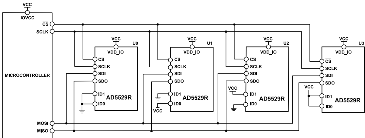
Figure 68. AD5529R WLCSP Daisy-Chain Configuration
