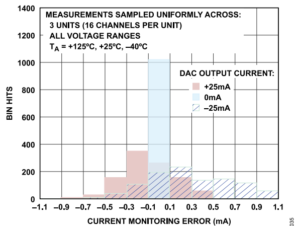
Figure 35. DAC Output Current Monitoring Error, Histogram
