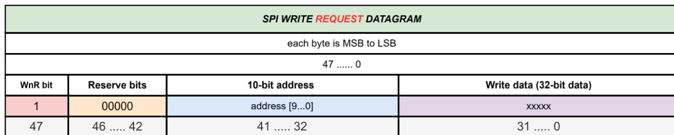
Figure 7. SPI Write Request Datagram Structure
