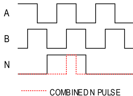
Figure 32. Typical ABN Encoder Signals and Combined N Pulse
