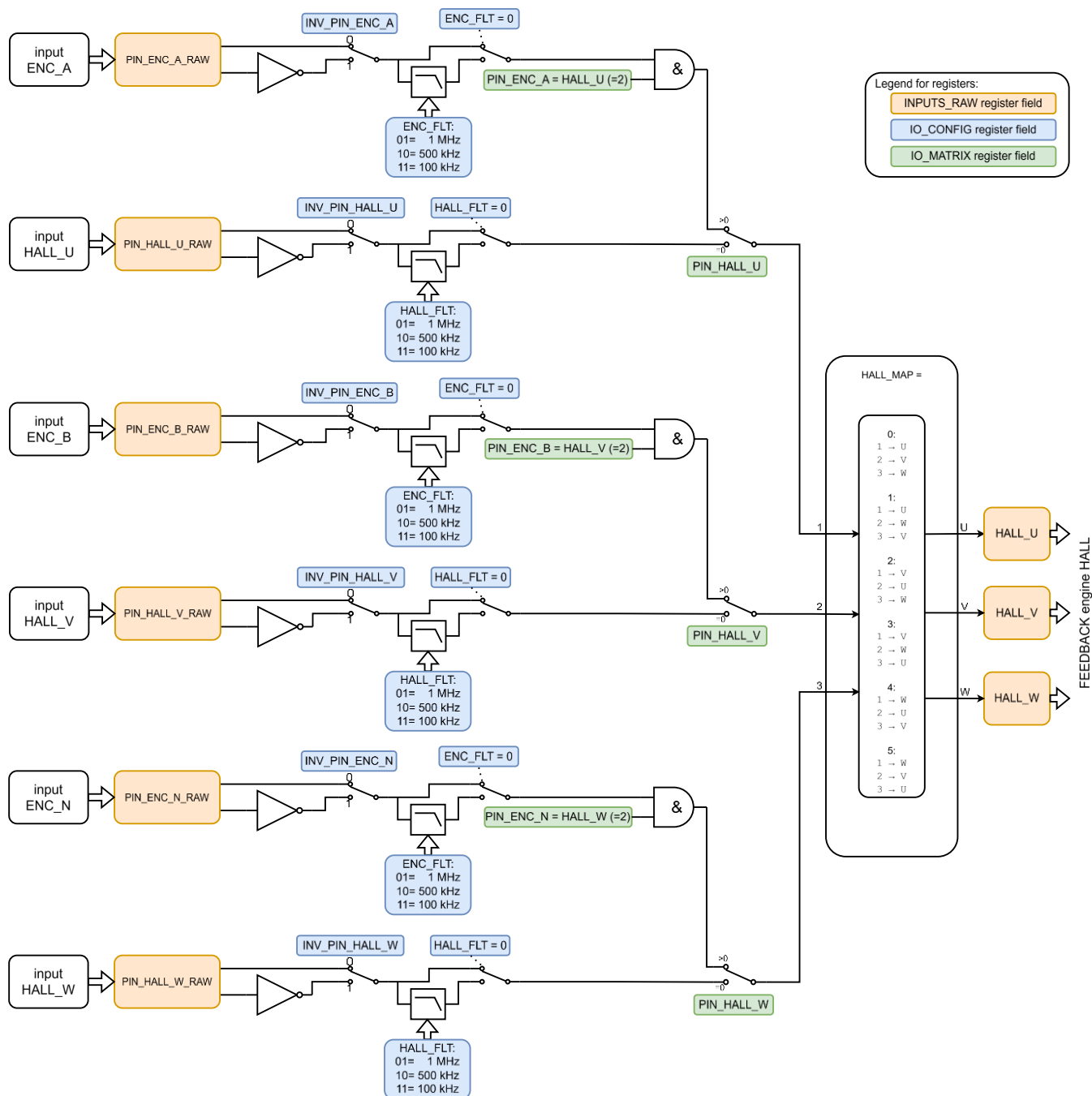
Figure 29. Digital Hall Feedback Configuration Options
