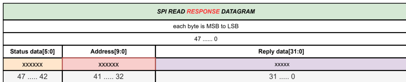
Figure 5. SPI Read Response Datagram Structure
