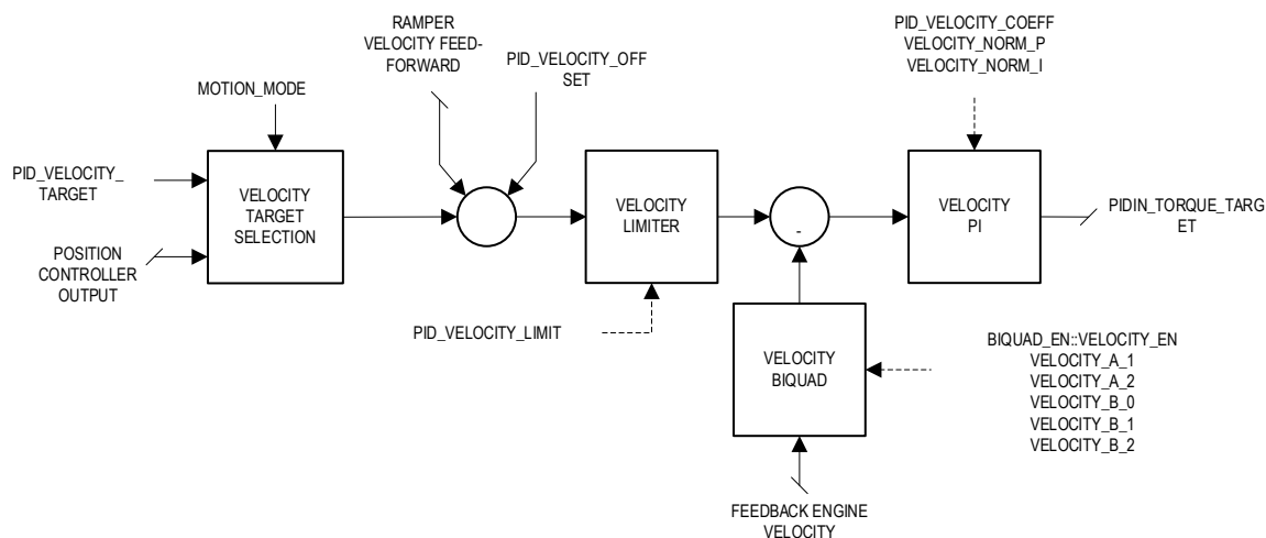
Figure 41. Velocity Control Loop.
