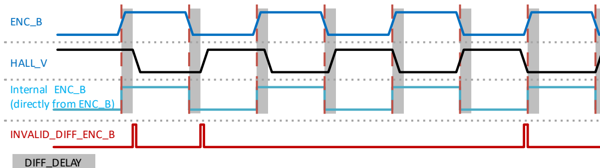
Figure 27. Digital Differential ABN Encoder Monitoring, Example for ENC_B vs. HALL_V Pins, DIFF_DELAY is Active after ENC_B Switches.
