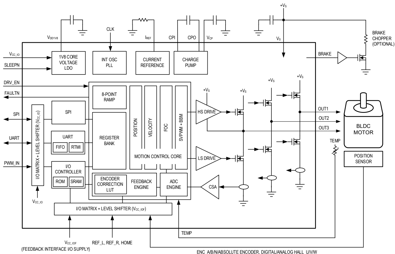
Figure 2. Functional Diagram
