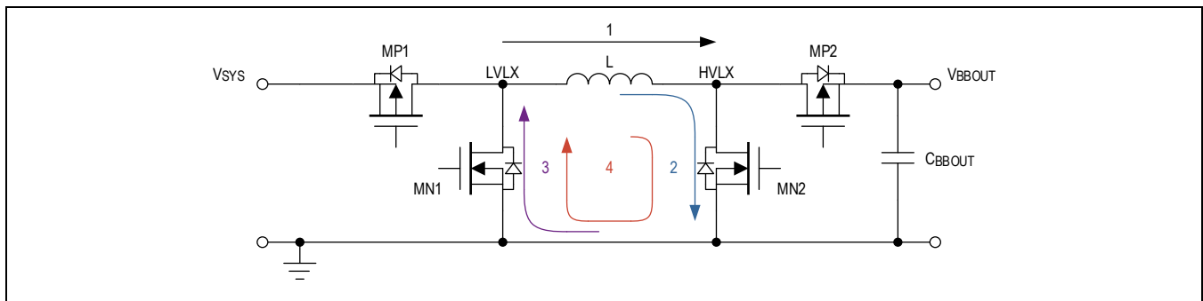
Figure 6. Buck-Boost Regulator and Switching Phases
