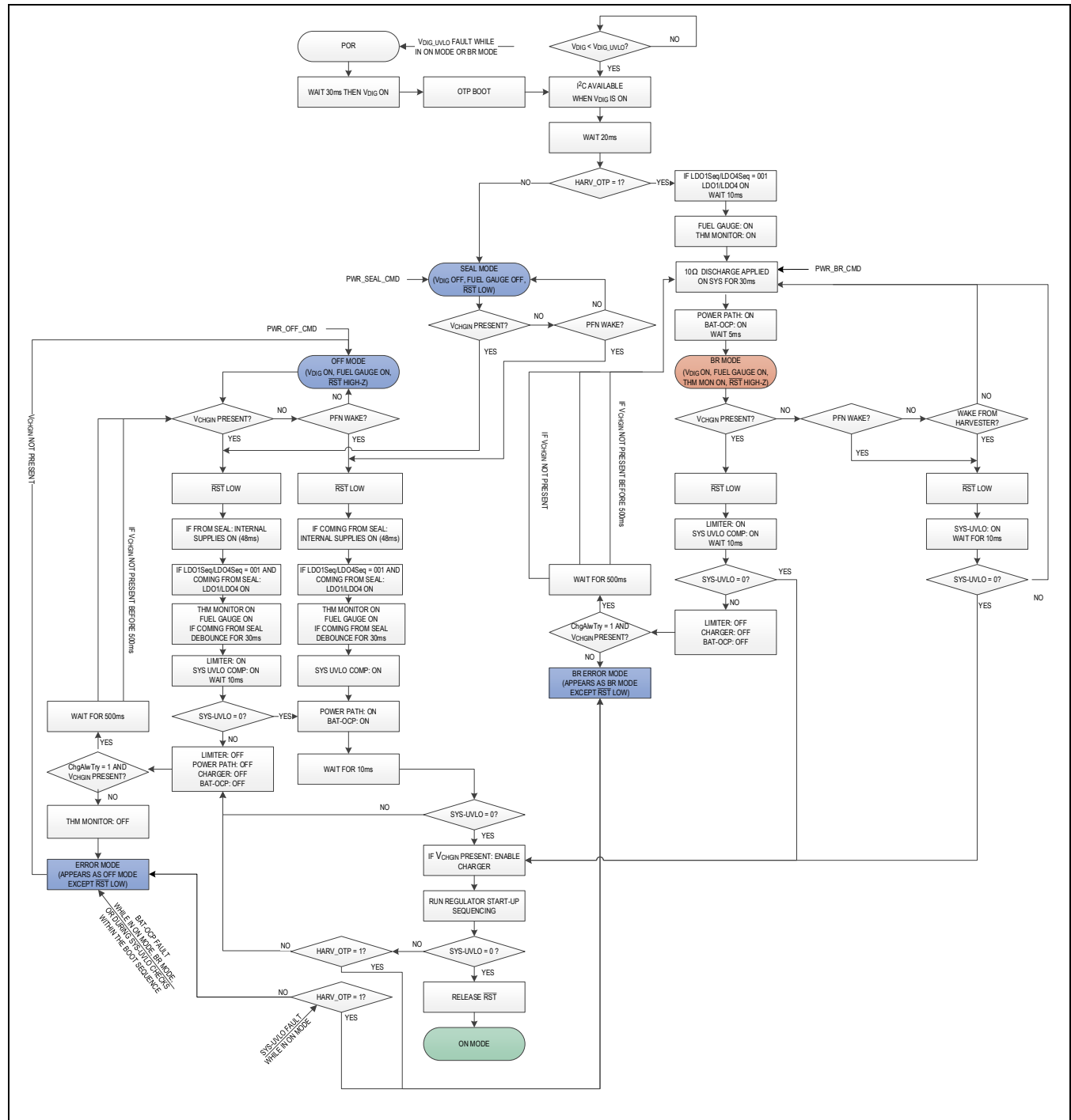
Figure 23. Boot Sequence—Harvester Mode Enabled
