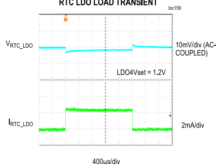
RTC LDO LOAD TRANSIENT
