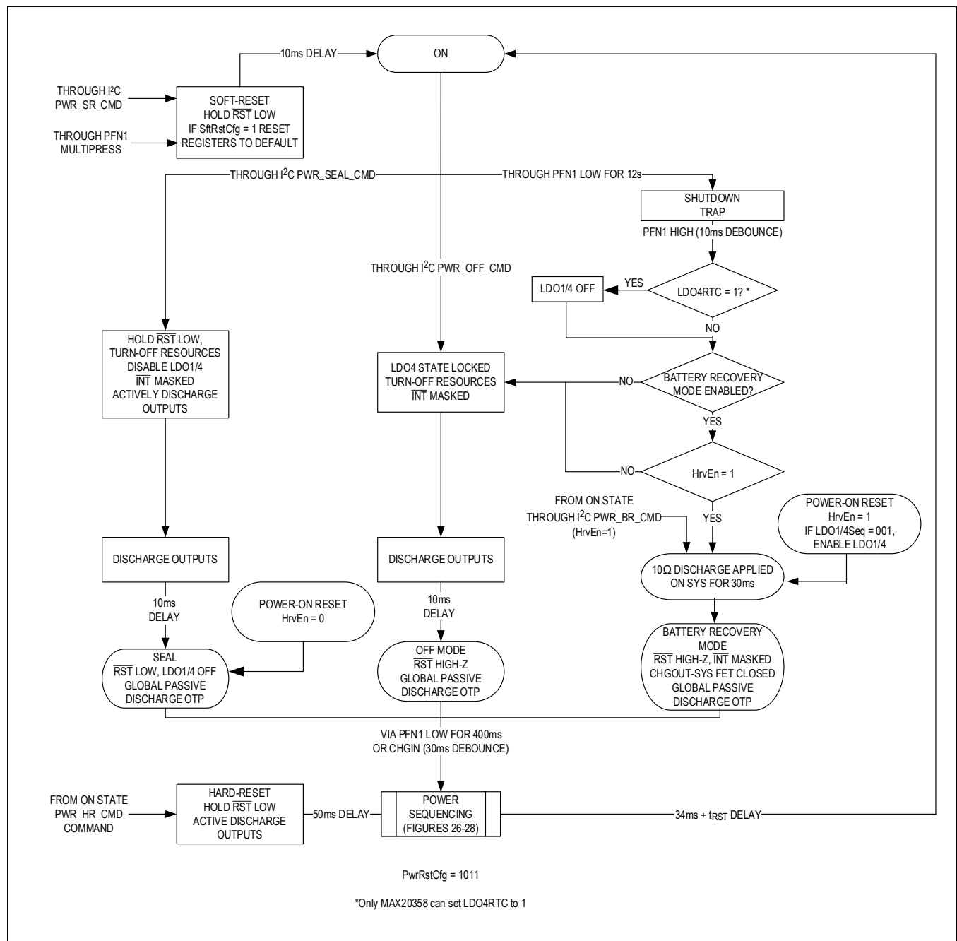
Figure 20. PwrRstCfg 1011
