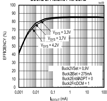
BUCK2 EFFICIENCY vs. LOAD
