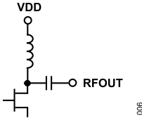
Figure 6. RFOUT and VDD Interface Schematic
