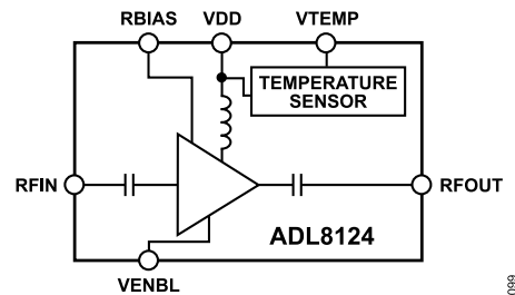
Figure 99. Simplified Architecture
