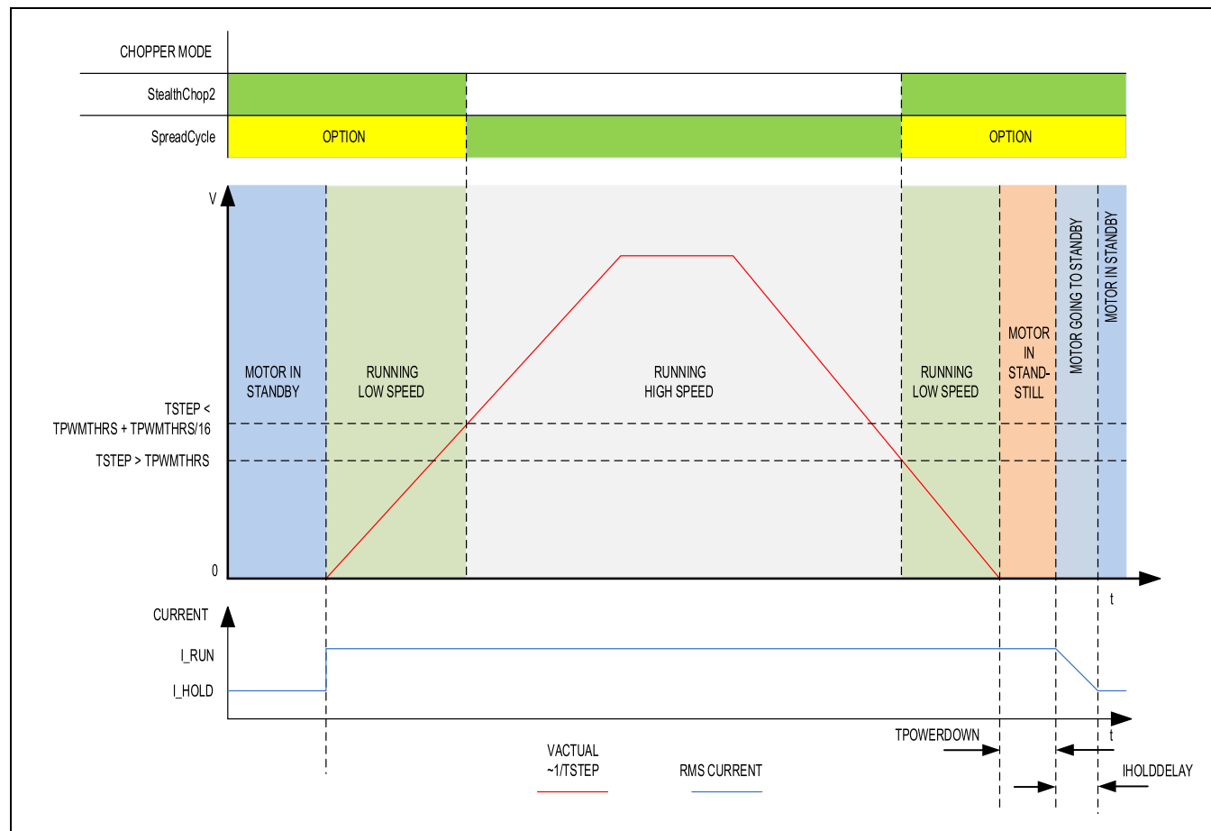
Figure 13. TPWMTHRS for Optional Switching to SpreadCycle
