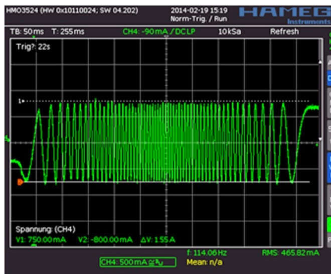
Figure 8. StealthChop2: Good Setting for PWM_REG
