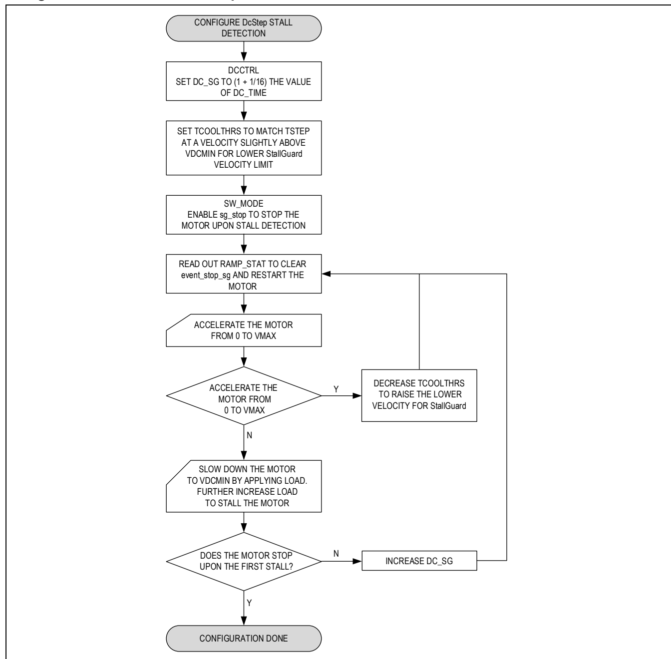
Figure 49. Quick Configuration Guide for Using Stall Detection with DcStep
