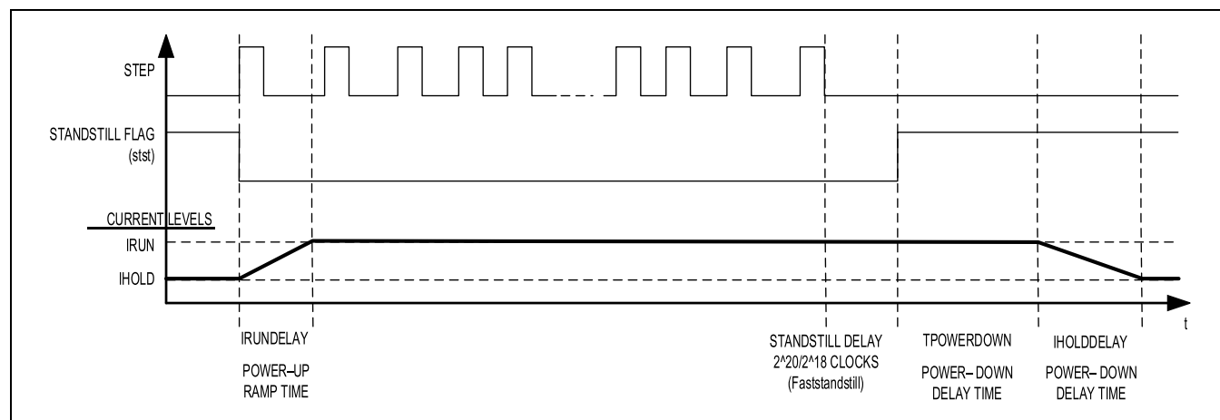
Figure 4. Automatic Motor Current Control at Standstill and Ramp-Up
