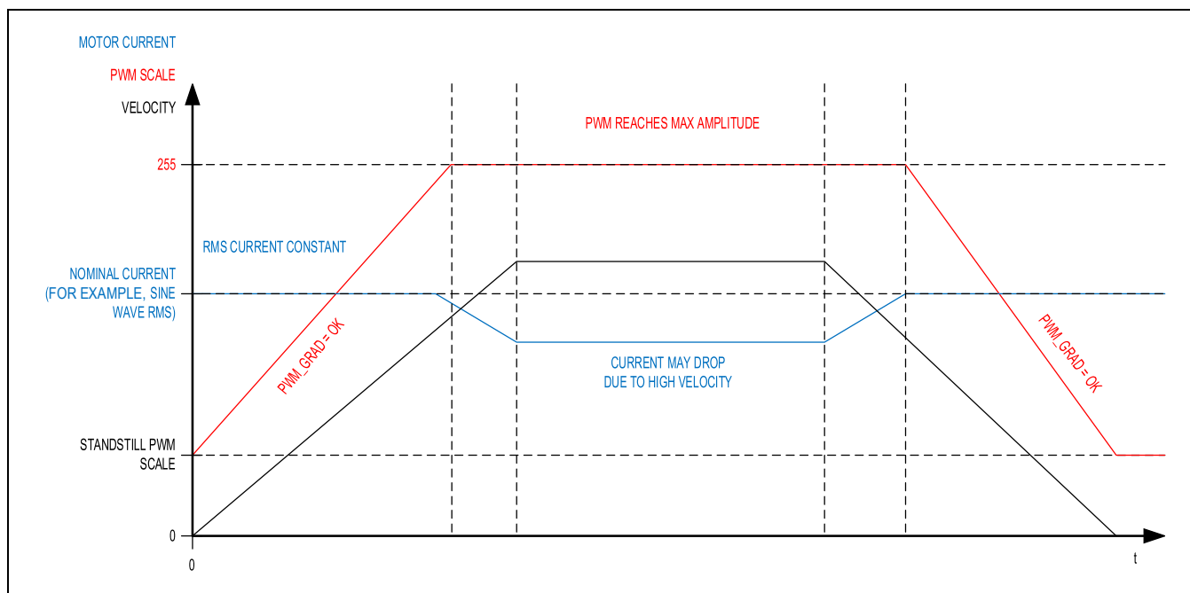
Figure 10. Successfully Determined PWM_GRAD(_AUTO) and PWM_OFS(_AUTO)
