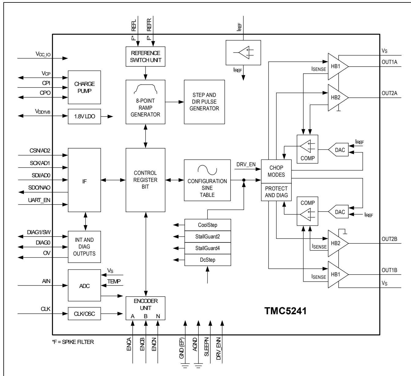
Figure 1. Block Diagram
