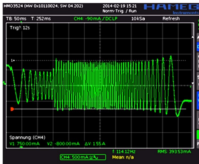
Figure 9. StealthChop2: Too Small Setting for PWM_REG during AT#2
