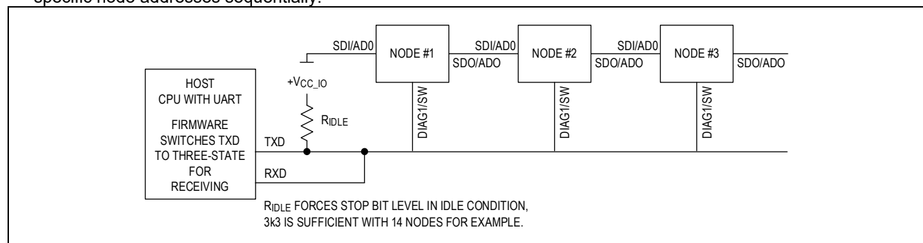
Figure 6. UART Daisy-Chaining Example
