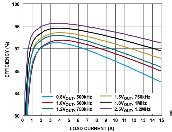
Figure 5. Efficiency, V_{IN} = 5\text{V} , V_{BIAS} = 3.3\text{V}
