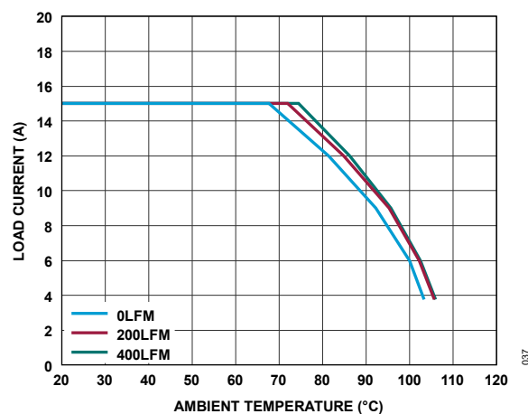
Figure 37. Derating Curve, No Heat Sink, V_{IN} = 12V , V_{OUT} = 3.3V , f_{SW} = 1.2MHz
