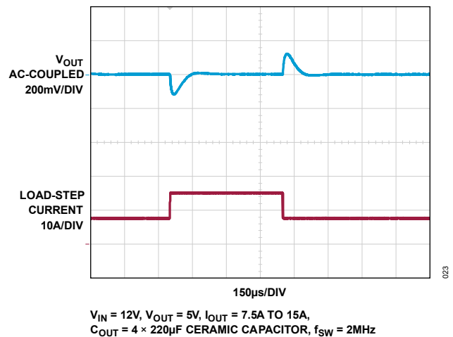
Figure 23. Output Transient Response, 5V
