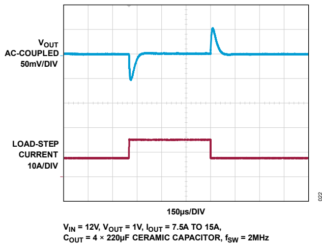
Figure 22. Output Transient Response, 1V
