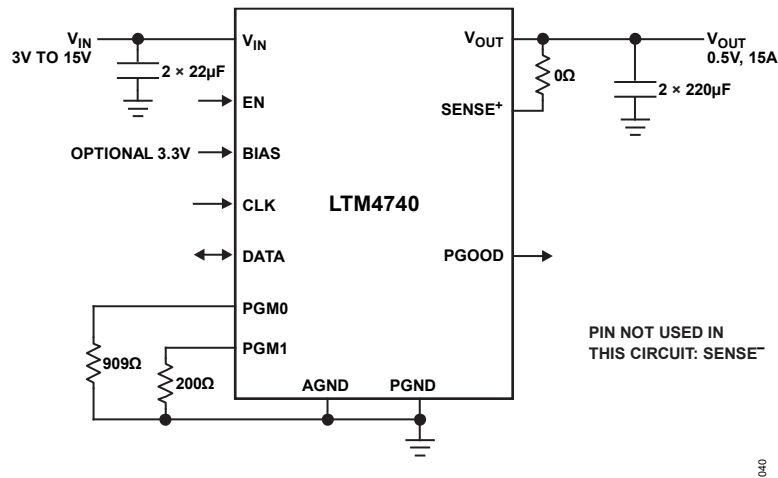
Figure 40. 0.5V, 15A Load from 3V to 15V Input, 500kHz Switching Frequency Design
