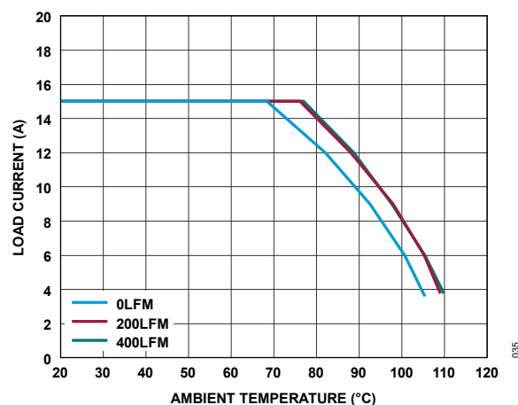
Figure 35. Derating Curve, No Heat Sink, V_{IN} = 12V , V_{OUT} = 2.5V , f_{SW} = 1.2MHz
