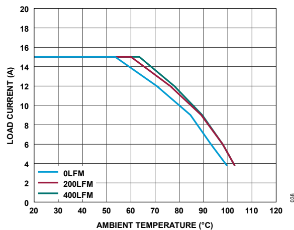
Figure 38. Derating Curve, No Heat Sink, V_{IN} = 12V , V_{OUT} = 5V , f_{SW} = 2MHz
