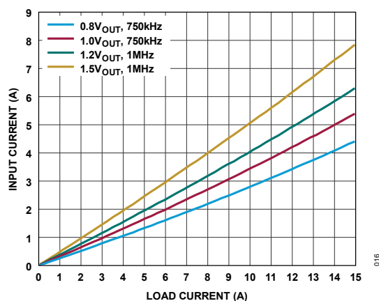
Figure 16. Input Current, V_{IN} = 3.3V , V_{BIAS} = 3.3V
