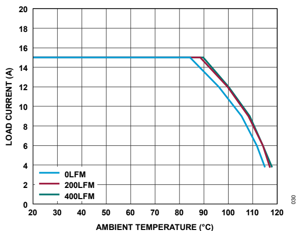
Figure 30. Derating Curve, No Heat Sink, V_{IN} = 5V , V_{OUT} = 1V , f_{SW} = 500kHz
