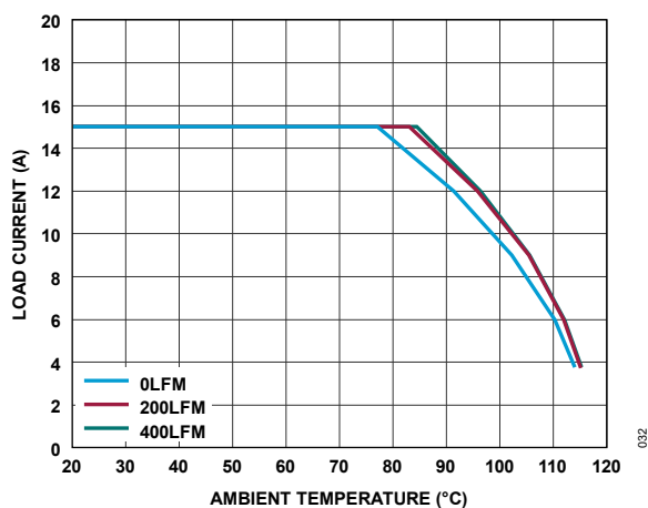
Figure 32. Derating Curve, No Heat Sink, V_{IN} = 5V , V_{OUT} = 1.8V , f_{SW} = 1MHz
