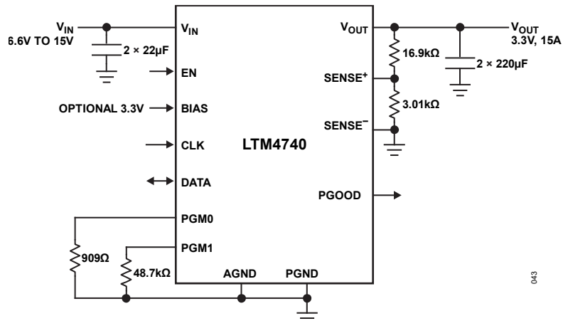
Figure 43. 3.3V Output, 15A Load from 6.6V to 15V Input, 1.2MHz Switching Frequency Design
