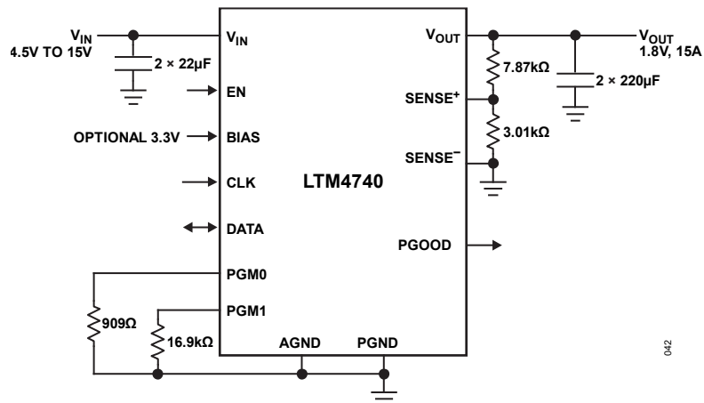
Figure 42. 3. 1.8V, 15A Load from 4.5V to 15V Input, 1MHz Switching Frequency Design
