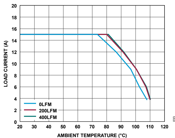
Figure 33. Derating Curve, No Heat Sink, V_{IN} = 12V , V_{OUT} = 1.8V , f_{SW} = 1MHz
