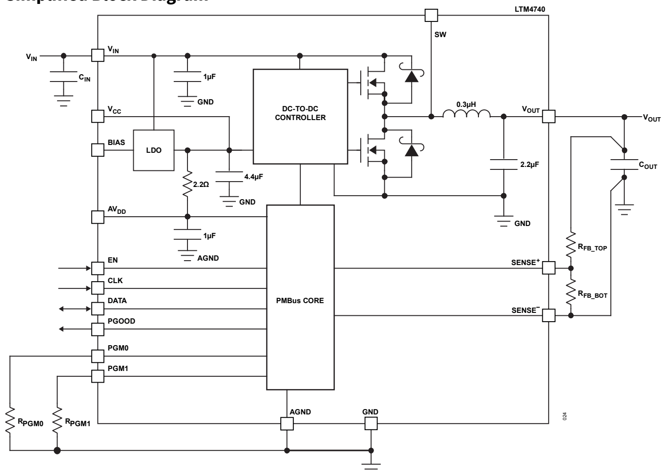
Figure 24. LTM4740 Simplified Block Diagram
