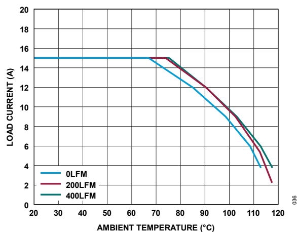
Figure 36. Derating Curve, No Heat Sink, V_{IN} = 5V , V_{OUT} = 3.3V , f_{SW} = 1.5MHz
