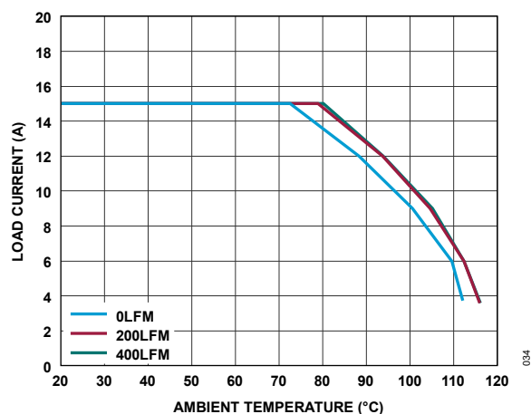
Figure 34. Derating Curve, No Heat Sink, V_{IN} = 5V , V_{OUT} = 2.5V , f_{SW} = 1.2MHz
