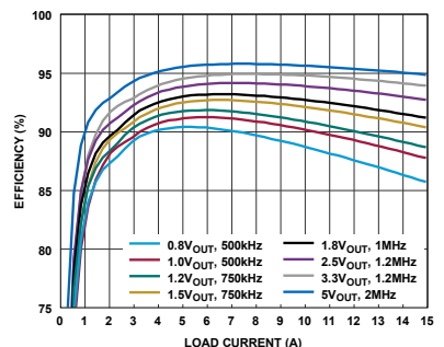
Figure 2. Efficiency, V IN = 12V, V BIAS = 3.3V
