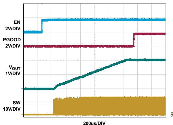
Figure 19. Startup without Pre-Bias
