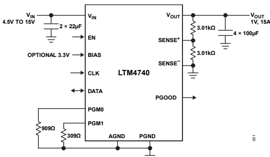
Figure 1. 4.5V to 15V Input to 1V, 15A Output
