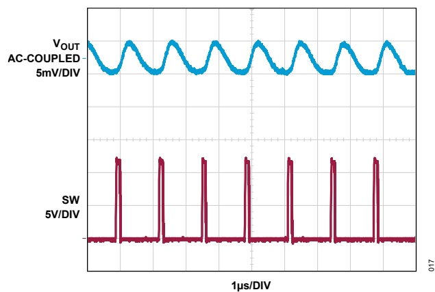
Figure 17. Output Voltage Ripple (FCM)
