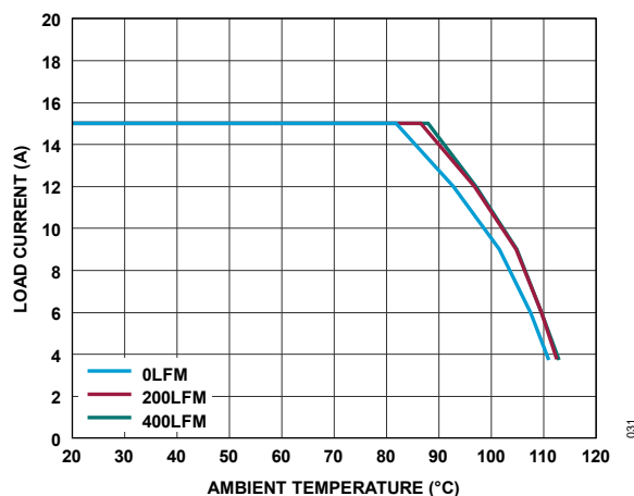
Figure 31. Derating Curve, No Heat Sink, V_{IN} = 12V , V_{OUT} = 1V , f_{SW} = 500kHz
