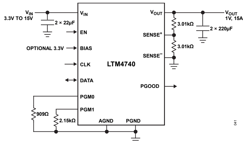
Figure 41. 1V, 15A Load from 3.3V to 15V Input, 750kHz Switching Frequency Design
