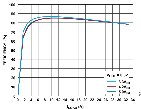
Figure 8. Efficiency vs. I_{LOAD} at Different V_{IN}
