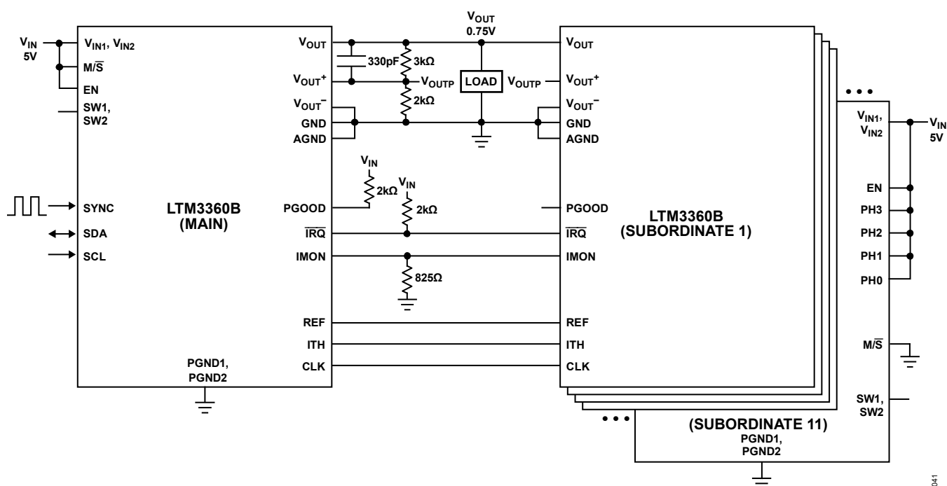
Figure 41. 12× LTM3360B (5V to 0.75V, 396A)
