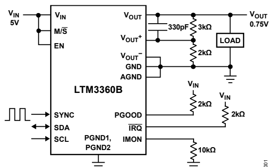
Figure 1. 5V to 0.75V at 33A, No Additional Capacitors
