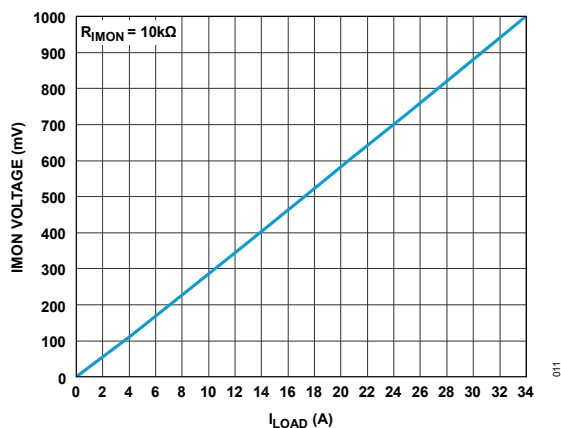
Figure 11. IMON Voltage vs. I_{LOAD}
