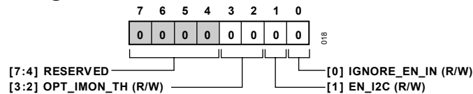
Figure 18. Address: 0x1, Reset: 0x00, Name: EN_IMON_CTRL
