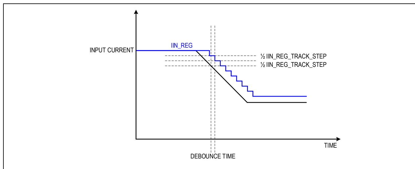
Figure 10. IIN_REG Auto Tracking
