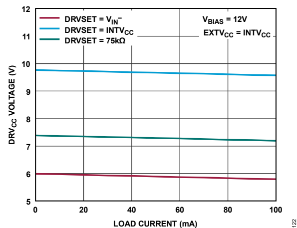
Figure 22. DRV CC Voltage vs. Load Current
