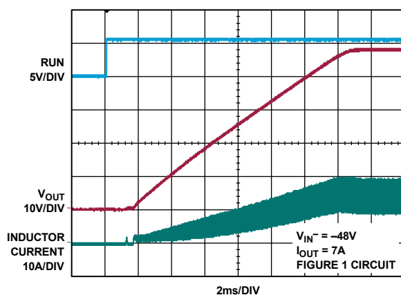
Figure 12. Soft Start-up
