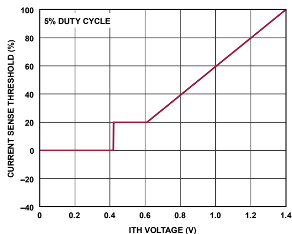
Figure 16. Maximum Current Sense Threshold Relative to V_{SENSE(MAX)} vs. V_{ITH} in Burst Mode
