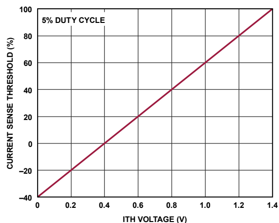
Figure 14. Maximum Current Sense Threshold Relative to V_{SENSE(MAX)} vs. V_{ITH} in Forced Continuous Mode
