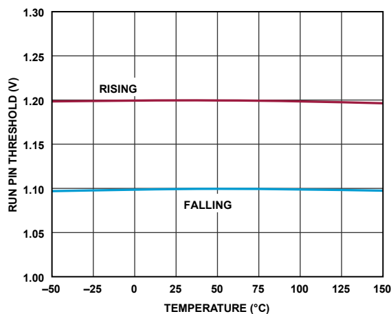
Figure 21. RUN Pin Thresholds vs. Temperature
