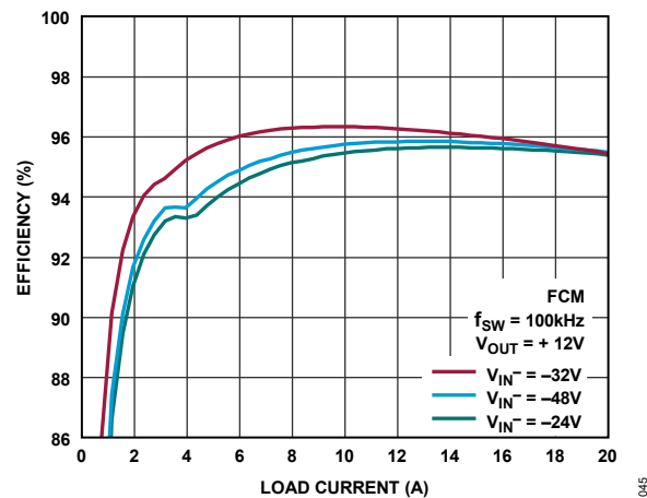
Figure 45. V_{OUT} Efficiency vs. Load Current for Figure 44
