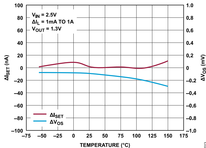
Figure 13. \Delta I_{\text{SET}} and \Delta V_{\text{OS}} Load Regulation vs. Temperature
