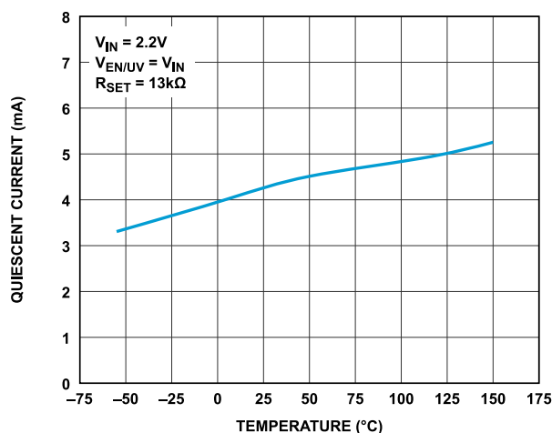
Figure 14. Quiescent Current vs. Temperature ( V_{\text{EN/UV}} = V_{\text{IN}} )
