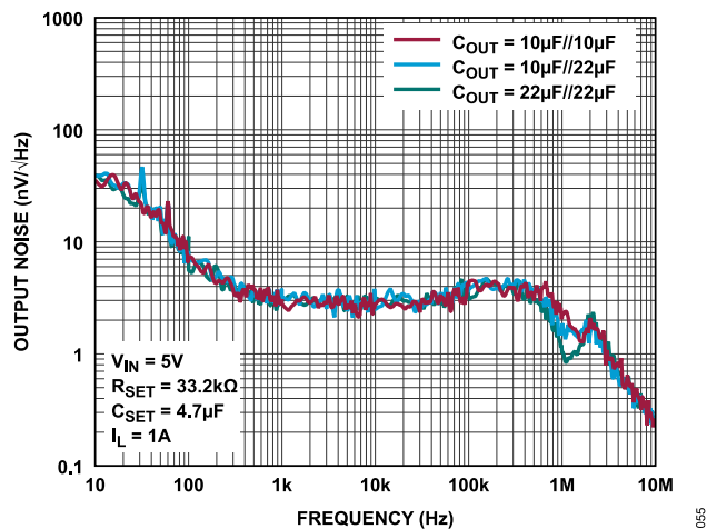
Figure 55. Output Noise vs. Frequency ( C_{OUT} Steps)
