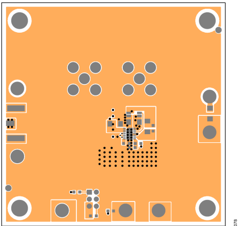
Figure 78. Recommended Layout
