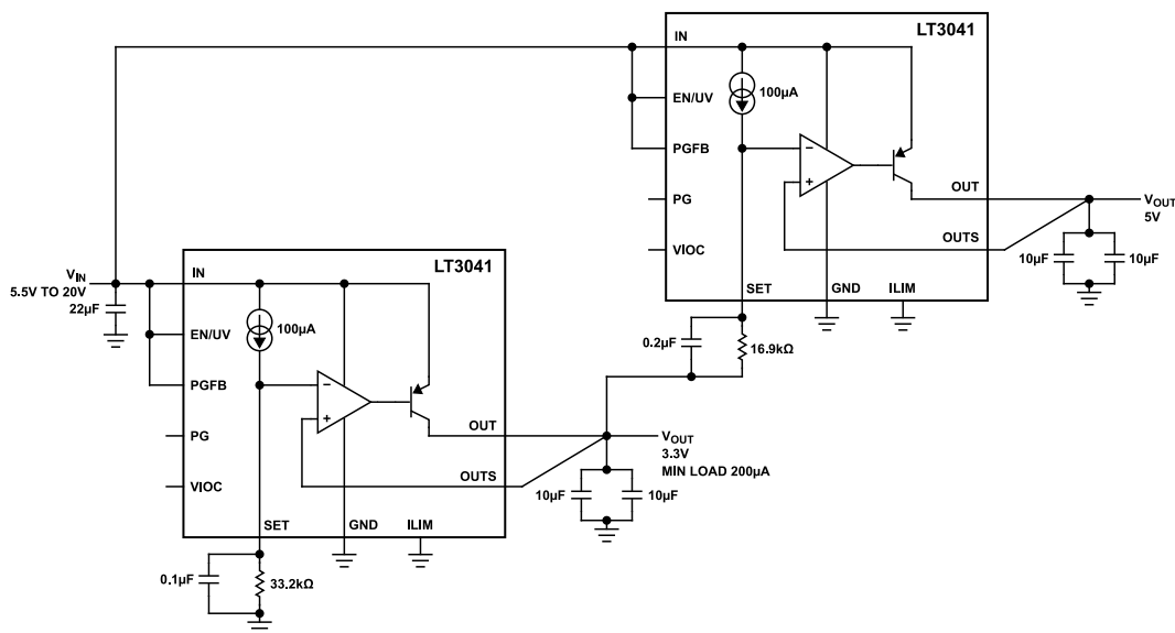
Figure 90. Ratiometric Tracking
