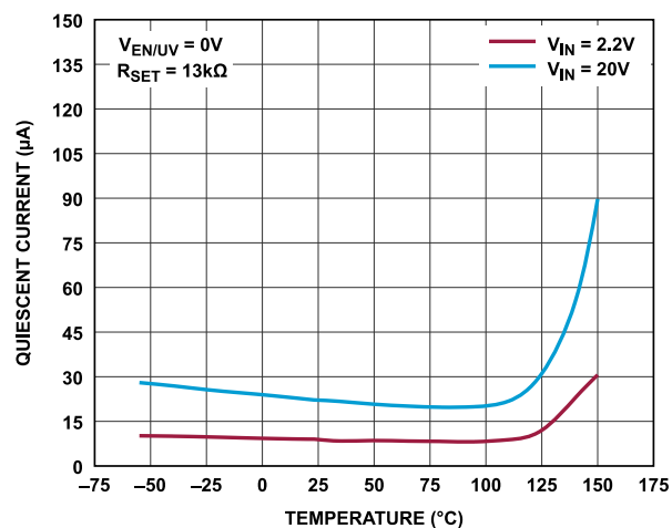
Figure 15. Quiescent Current vs. Temperature ( V_{\text{EN/UV}} = 0 \text{ V} )
