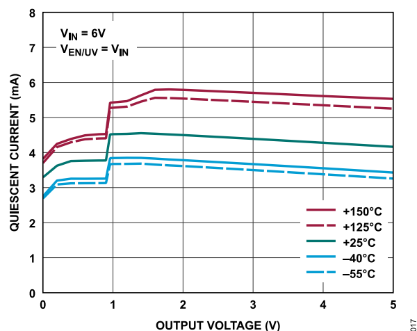
Figure 17. Quiescent Current vs. Output Voltage
