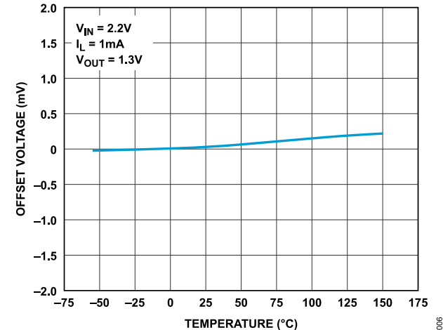
Figure 6. Offset Voltage ( V_{OUT} - V_{SET} ) vs. Temperature
