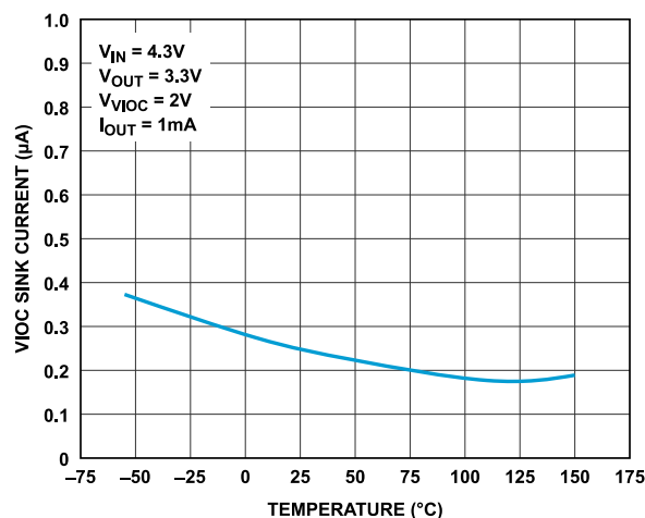
Figure 68. VIOC Sink Current vs. Temperature
