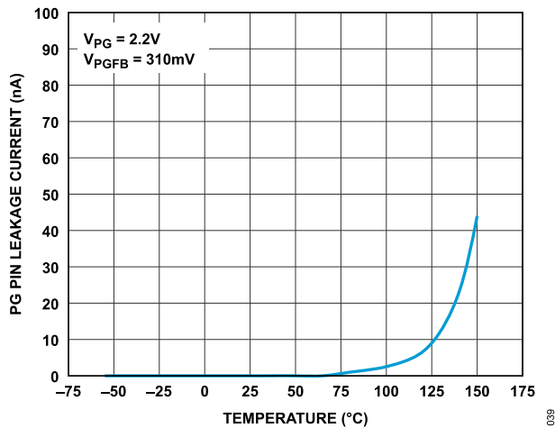
Figure 39. PG Pin Leakage Current vs. Temperature
