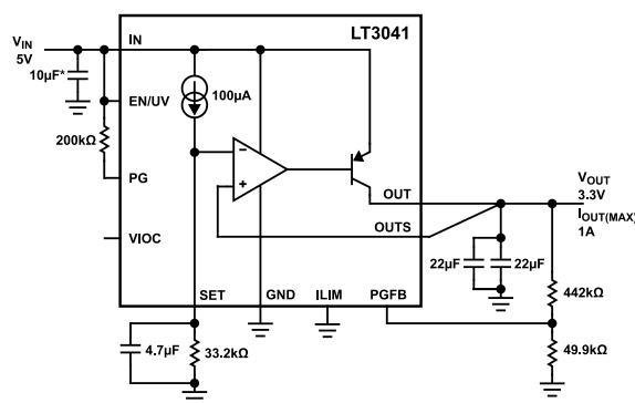
Figure 1. Typical Application
