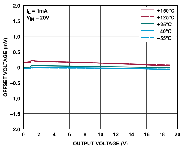
Figure 11. Offset Voltage ( V_{\text{OUT}} - V_{\text{SET}} ) vs. Output Voltage
