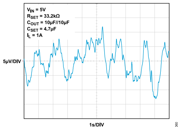
Figure 60. Output Noise: 0.1 Hz to 10 Hz (CSET = 4.7 μF)
