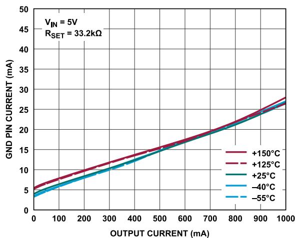
Figure 21. GND Pin Current vs. Output Current
