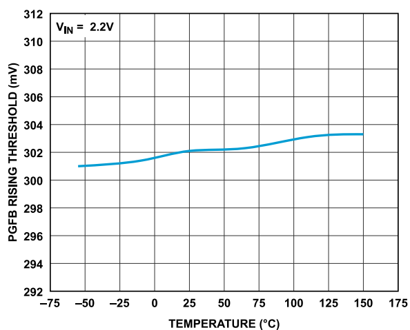
Figure 36. PGFB Rising Threshold vs. Temperature
