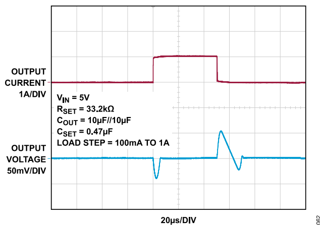
Figure 62. Load-Transient Response
