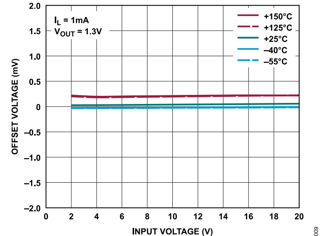
Figure 9. Offset Voltage ( V_{OUT} - V_{SET} ) vs. Input Voltage
