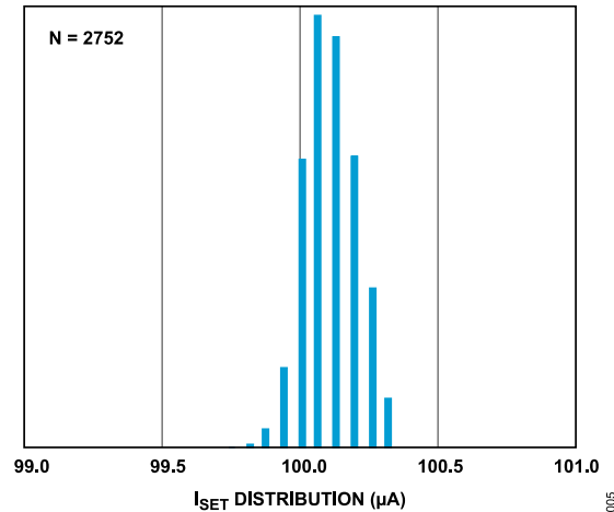
Figure 5. I_{SET} Distribution
