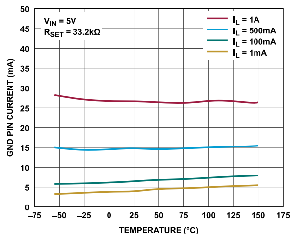
Figure 20. GND Pin Current vs. Temperature
