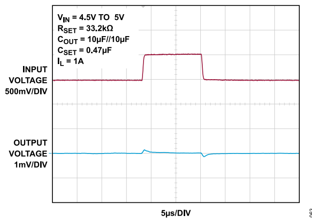
Figure 63. Line-Transient Response
