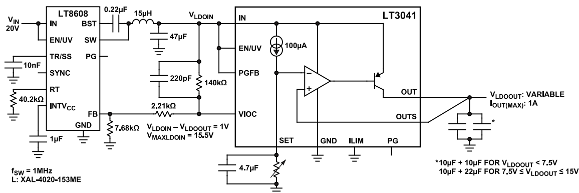
Figure 81. Typical LT3041 Post-Regulating Application
