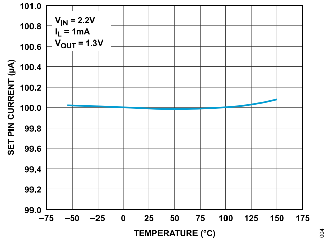
Figure 4. SET Pin Current vs. Temperature
