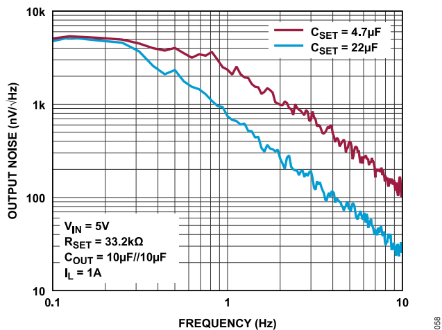
Figure 58. Output Noise (0.1 Hz to 10 Hz) vs. Frequency
