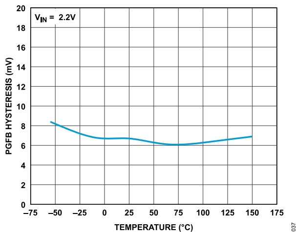
Figure 37. PGFB Hysteresis vs. Temperature
