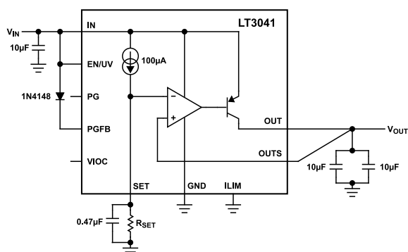
Figure 96. PGFB Disabled with Reverse-Input Protection
