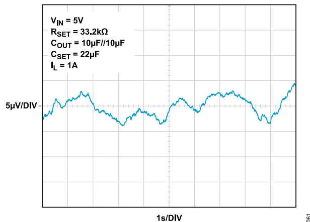
Figure 61. Output Noise: 0.1 Hz to 10 Hz (CSET = 22 μF)
