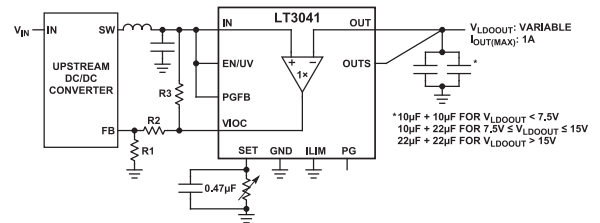
Figure 80. Programming Input-to-Output Differential
