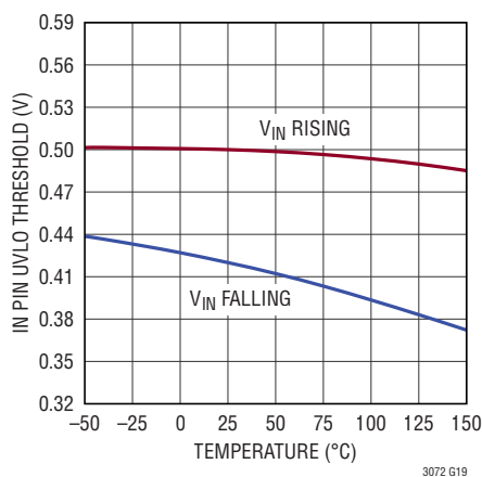
IN Pin Undervoltage Lockout Threshold
