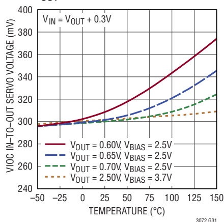
VIOC V_{IN} - V_{OUT} Servo Voltage, I_{OUT} = 2.5A
