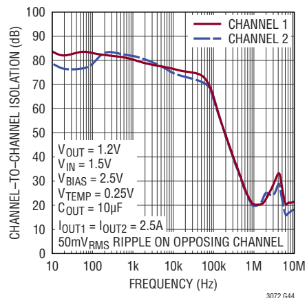
Channel-to-Channel Isolation
