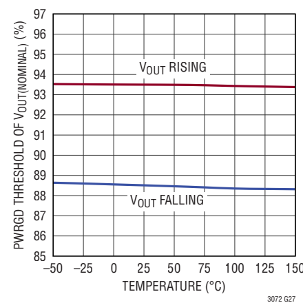
PWRGD Threshold
