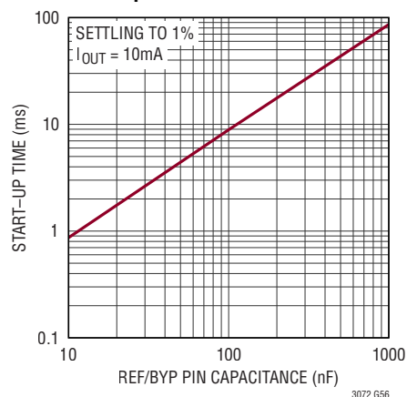
Start-Up Time
