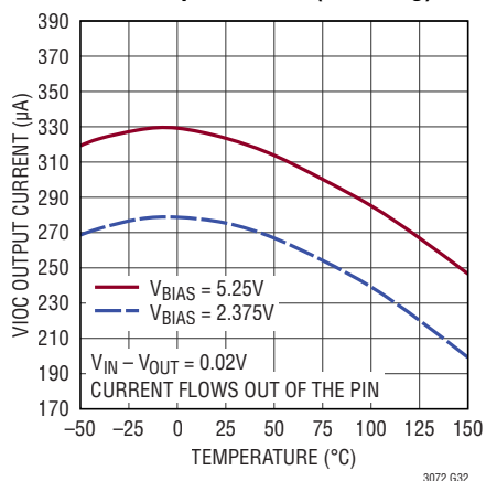
VIOC Output Current (Sourcing)
