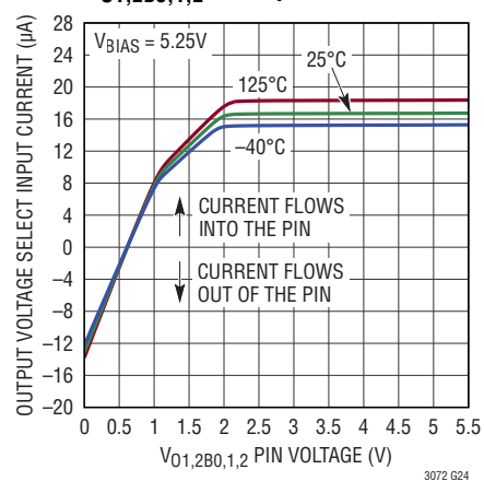
V_{O1,2B0,1,2} Pin Input Current
