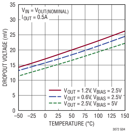
Dropout Voltage (0.5A)
