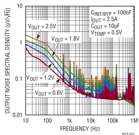
Output Noise Spectral Density vs V_{OUT}
