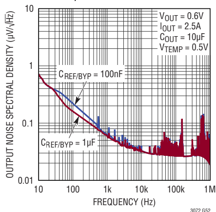
Output Noise Spectral Density vs C_{REF/BYP}
