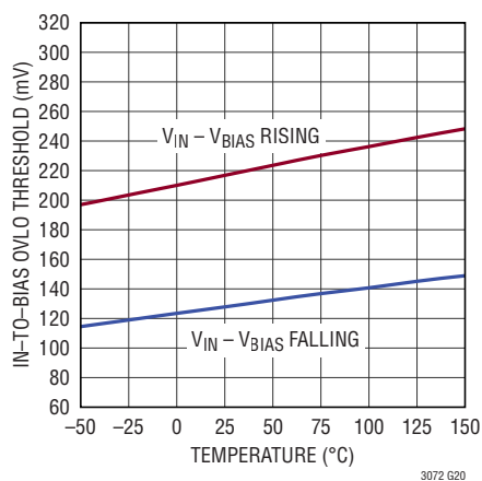
V_{IN} - V_{BIAS} Overvoltage Lockout Threshold
