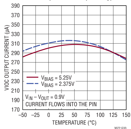
VIOC Output Current (Sinking)
