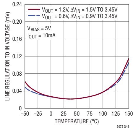
Line Regulation to V_{IN}
