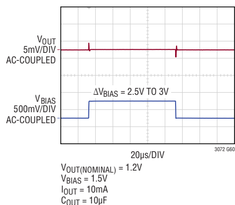
VBIAS Line Transient Response
