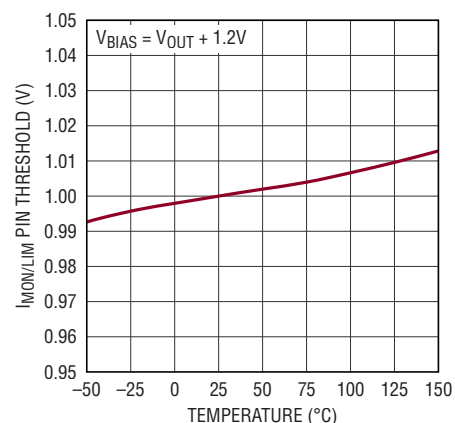
I_{MON}/I_{LM} External Current Limit Threshold
