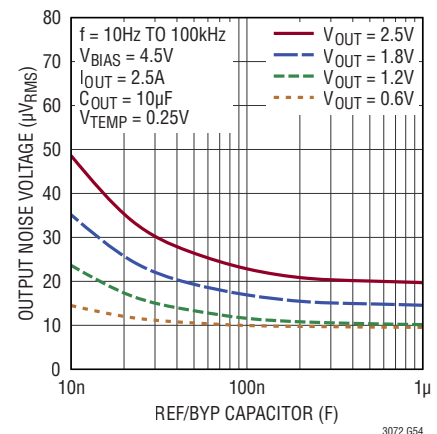
RMS Output Noise vs C_{REF/BYP}
