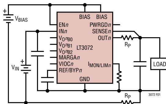
Figure 1. Kelvin Sense
