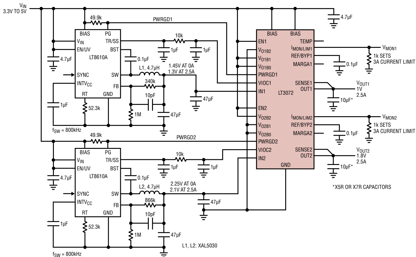
Dual Supply with Independent VOIC Buck Control
