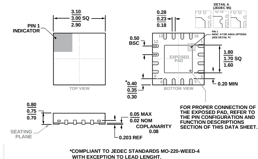
Figure 60. 16-Lead Lead Frame Chip Scale Package [LFCSP] 3 mm x 3 mm Body and 0.75 mm Package Height (CP-16-48) Dimensions shown in millimeters
