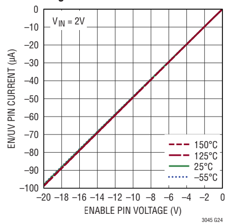
Negative Enable Pin Current
