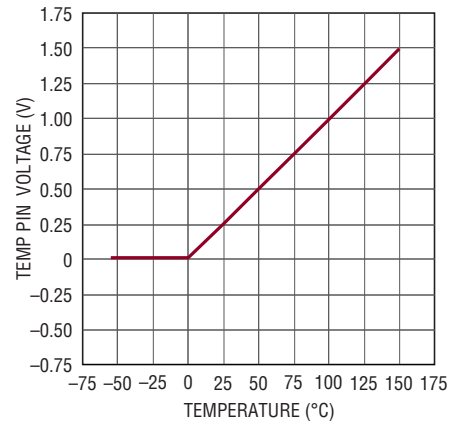
TEMP Output Voltage vs Temperature
