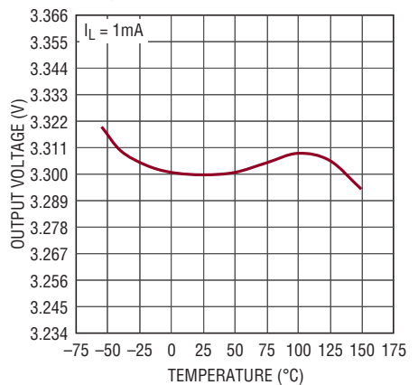
Output Voltage—LT3055-3.3
