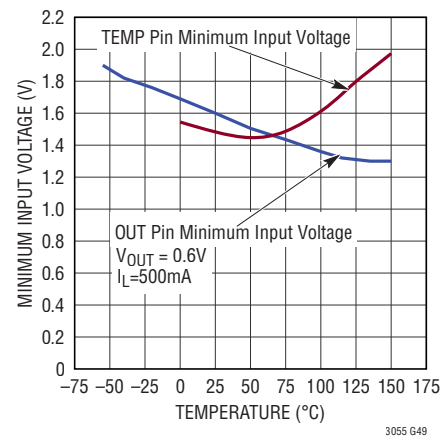
TEMP Pin Minimum Input Voltage
