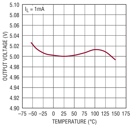
Output Voltage—LT3055-5
